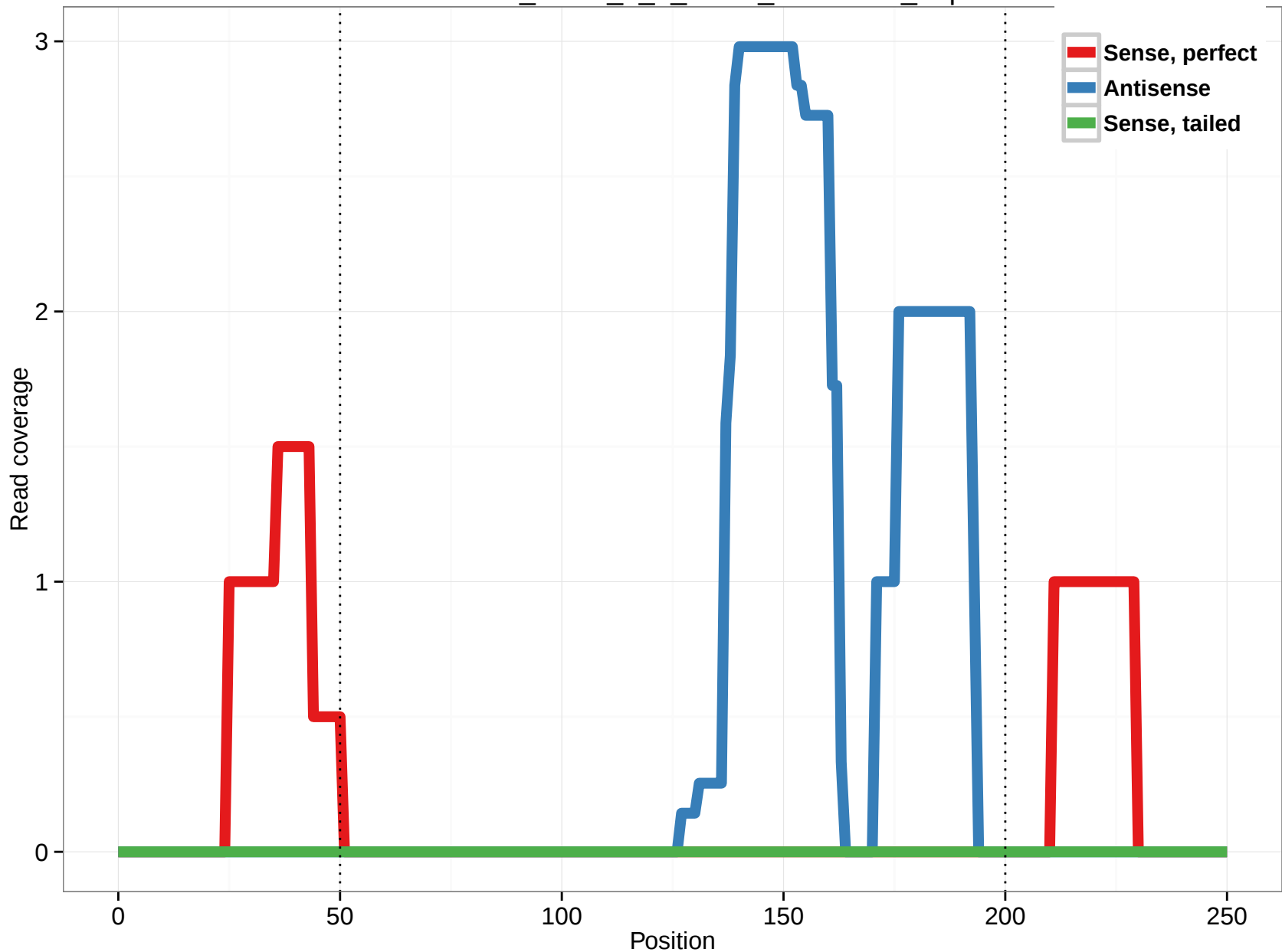
uc002die.2_intron_8_0_chr16_21145776_r.5p
