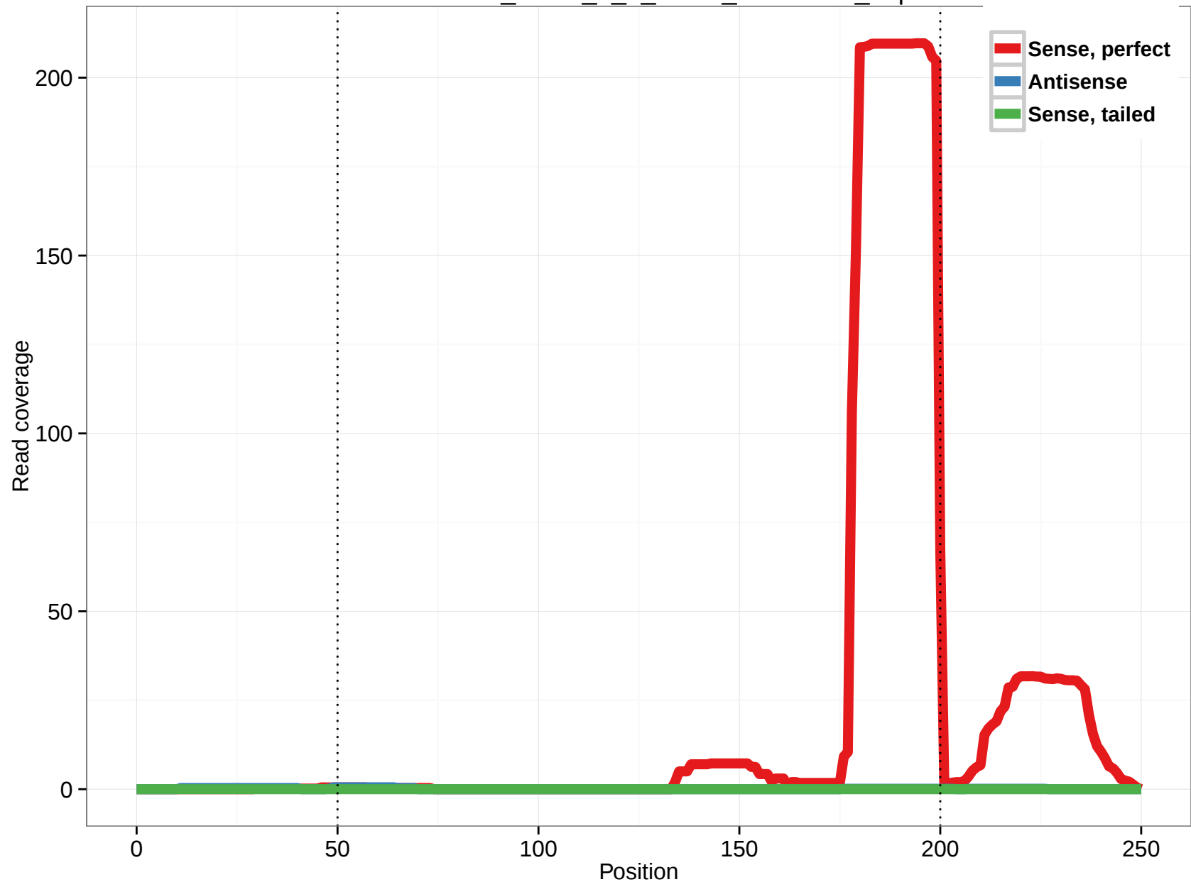
uc002dev.3_intron_5_0_chr16_16438310_f.3p
