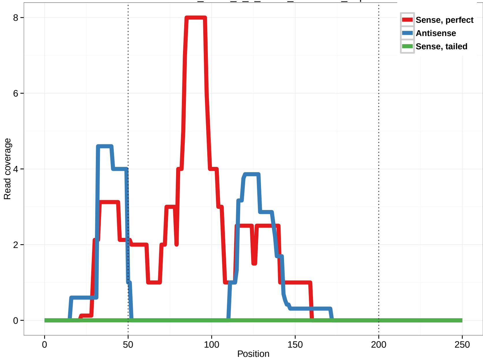
uc002dae.1_intron_2_0_chr16_10865656_r.3p
