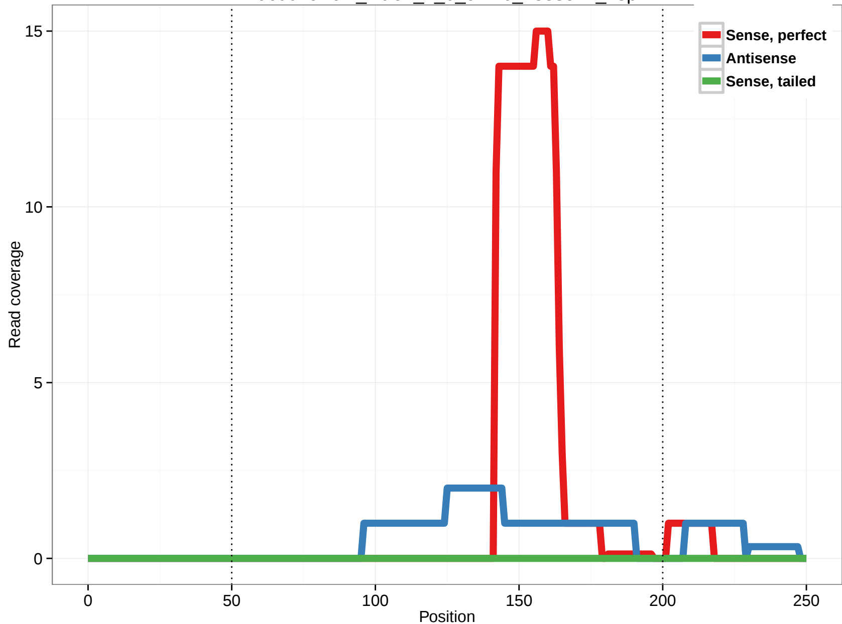
uc002cwc.1_intron_1_0_chr16_4383521_f.3p
