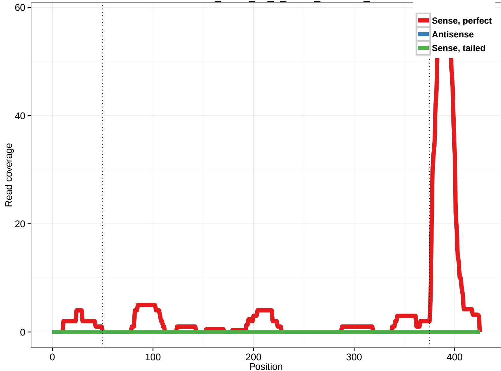
uc002cvv.2_intron_23_0_chr16_3830880_r
