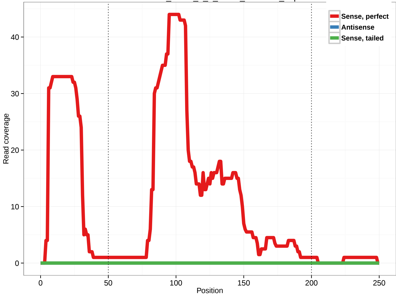
uc002cuv.3_intron_0_0_chr16_3358837_f.5p
