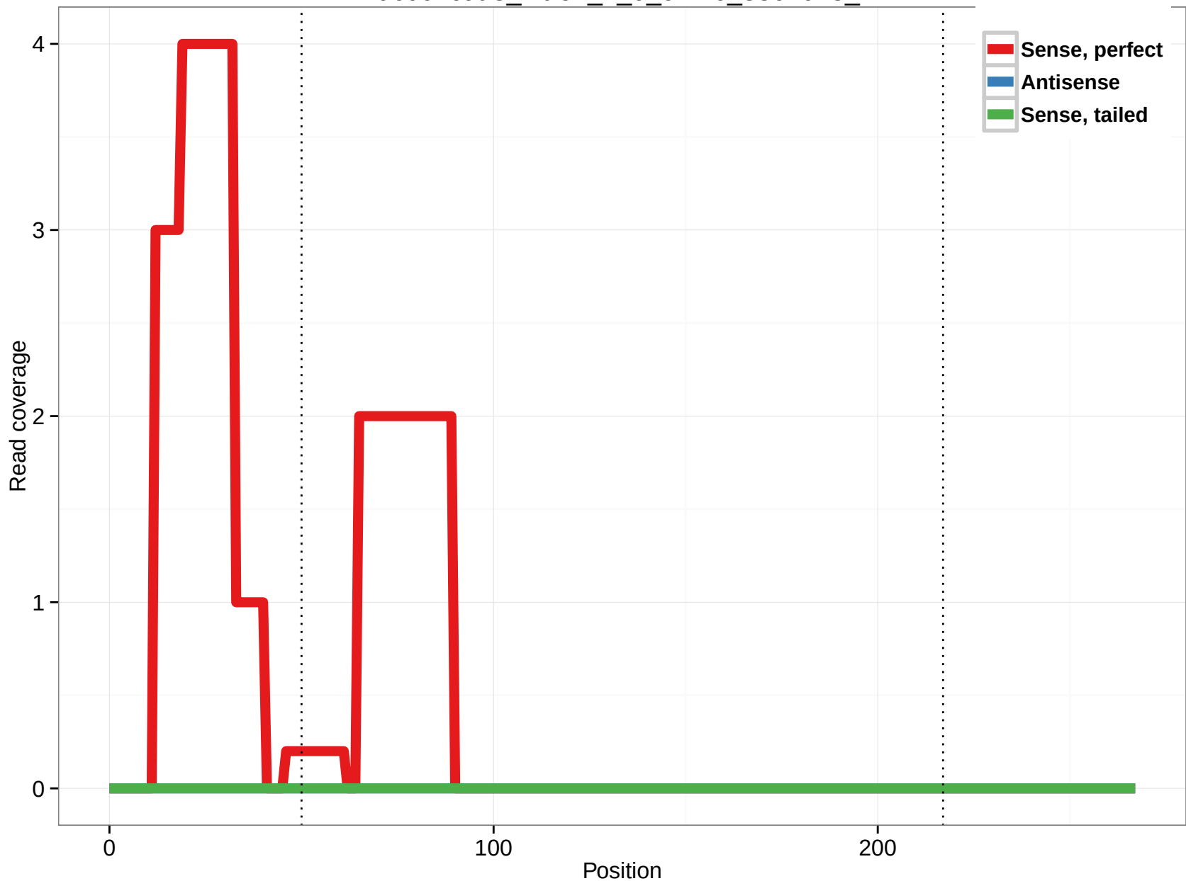
uc002cut.3_intron_4_0_chr16_3367023_f
