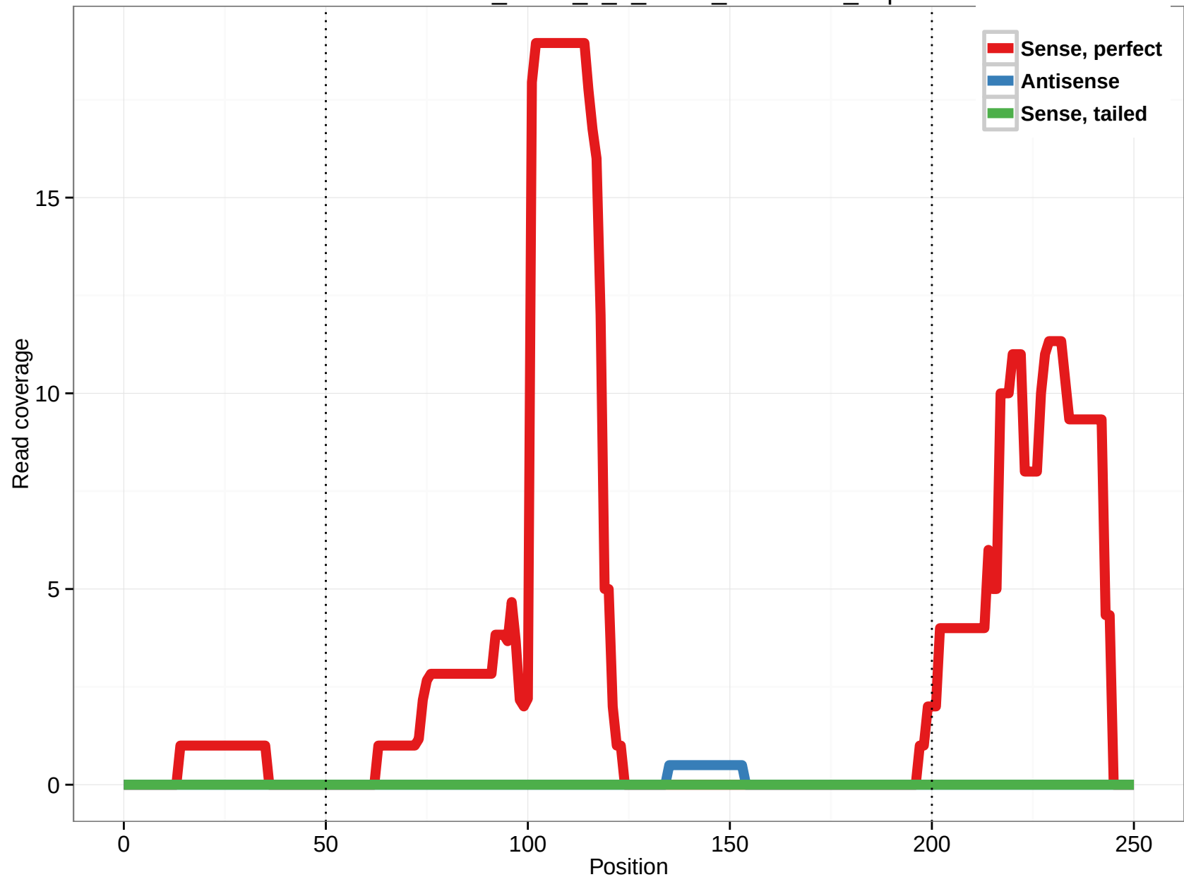
uc002bsn.2_intron_9_0_chr15_93487746_f.3p
