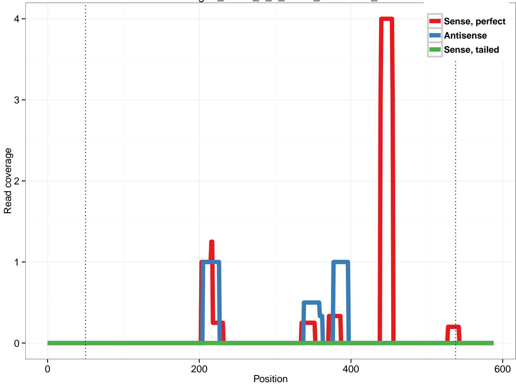
uc002bgr.2_intron_2_0_chr15_82385836_f
