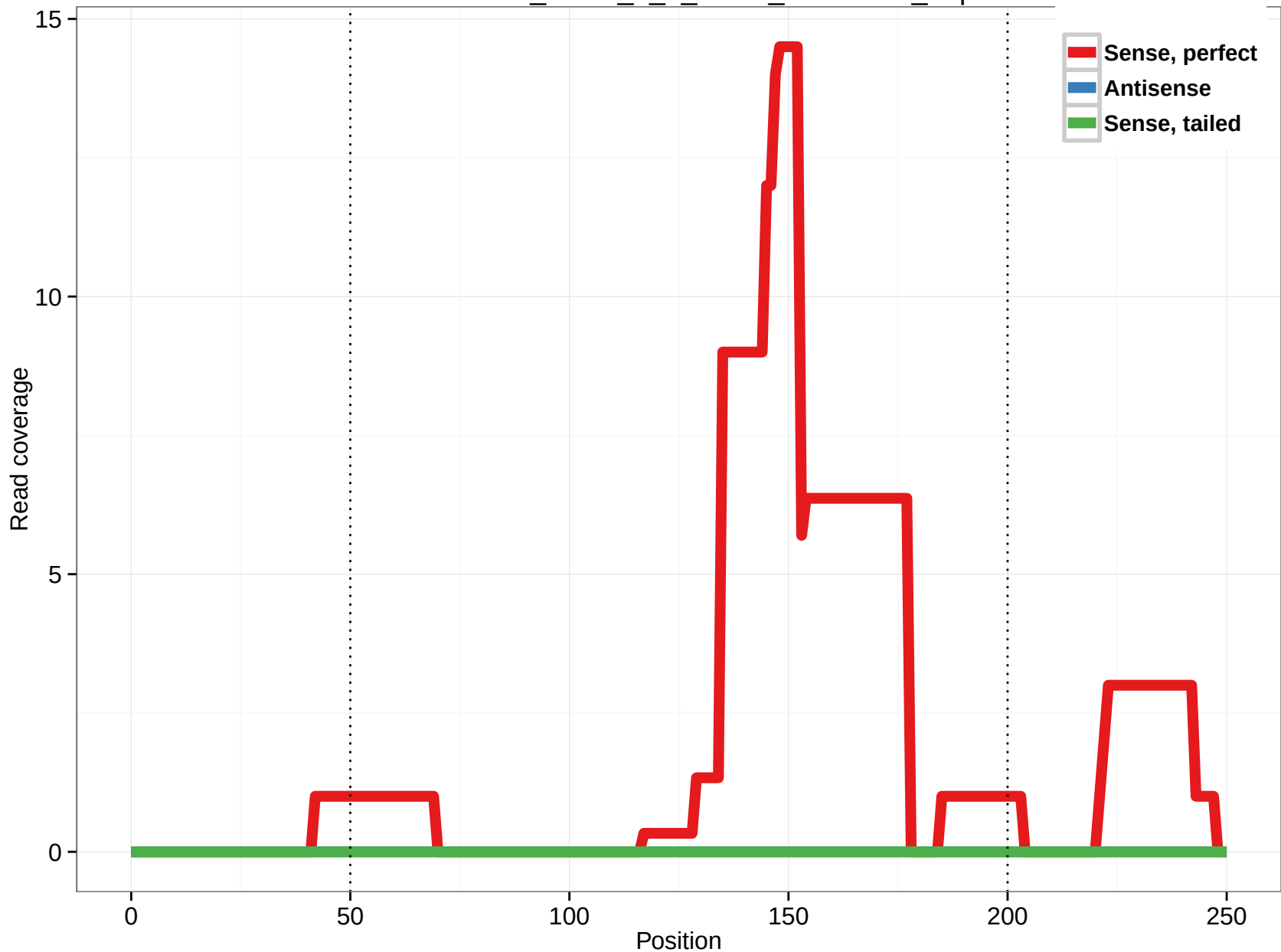
uc002bez.3_intron_1_0_chr15_80200027_r.3p
