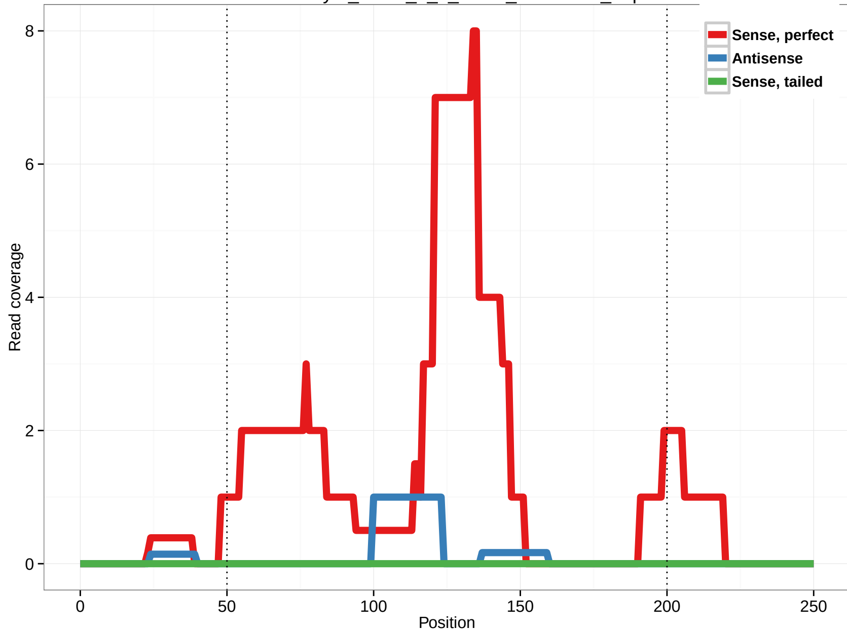
uc002bay.1_intron_1_0_chr15_76024494_r.5p
