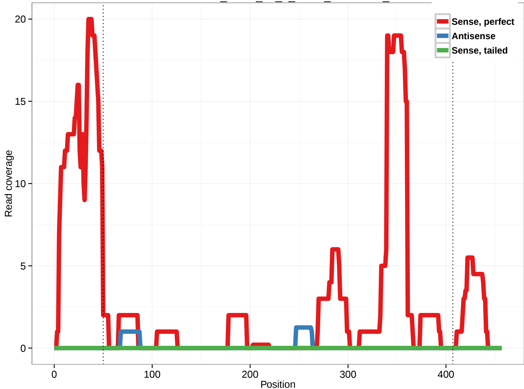
uc002baf.2_intron_13_0_chr15_75653030_r
