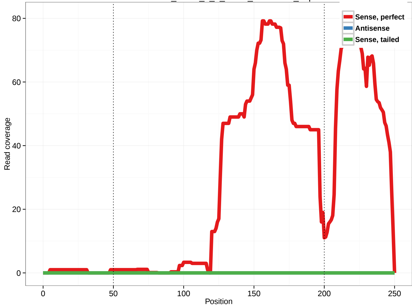
uc002asd.1_intron_1_0_chr15_69746061_f.3p
