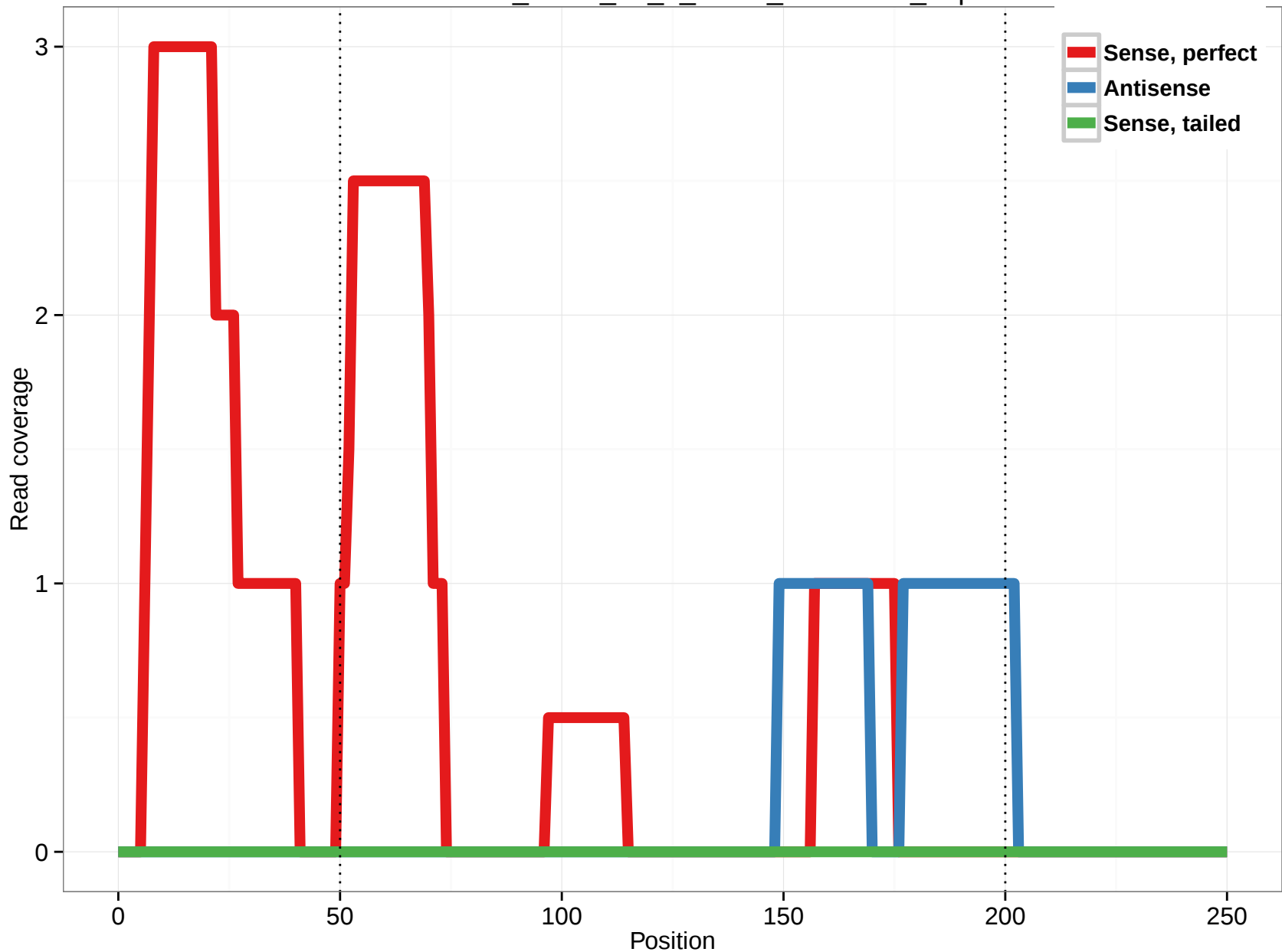
uc002ant.2_intron_10_0_chr15_65114810_r.5p
