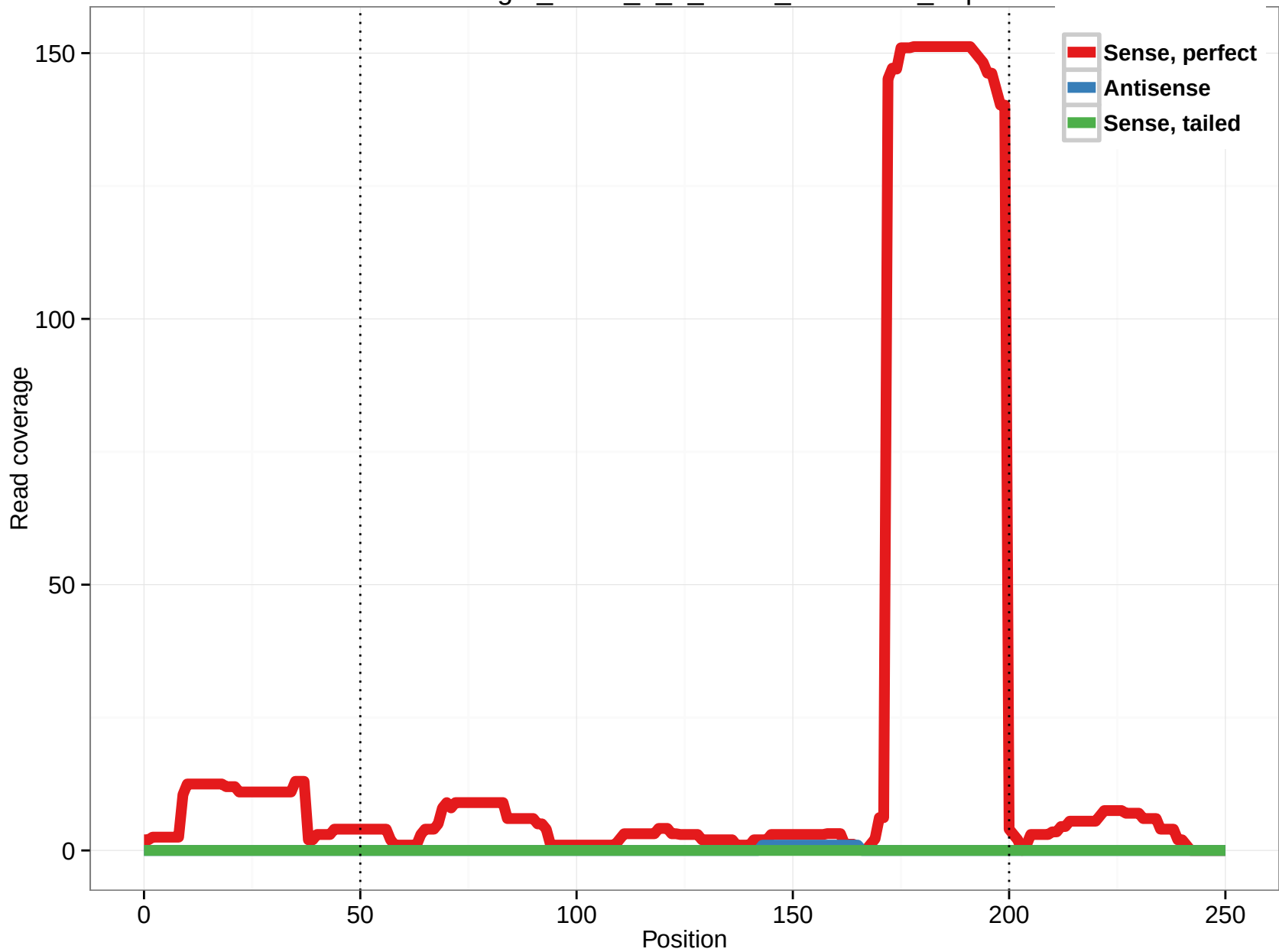
uc002ang.1_intron_0_0_chr15_64458280_r.3p
