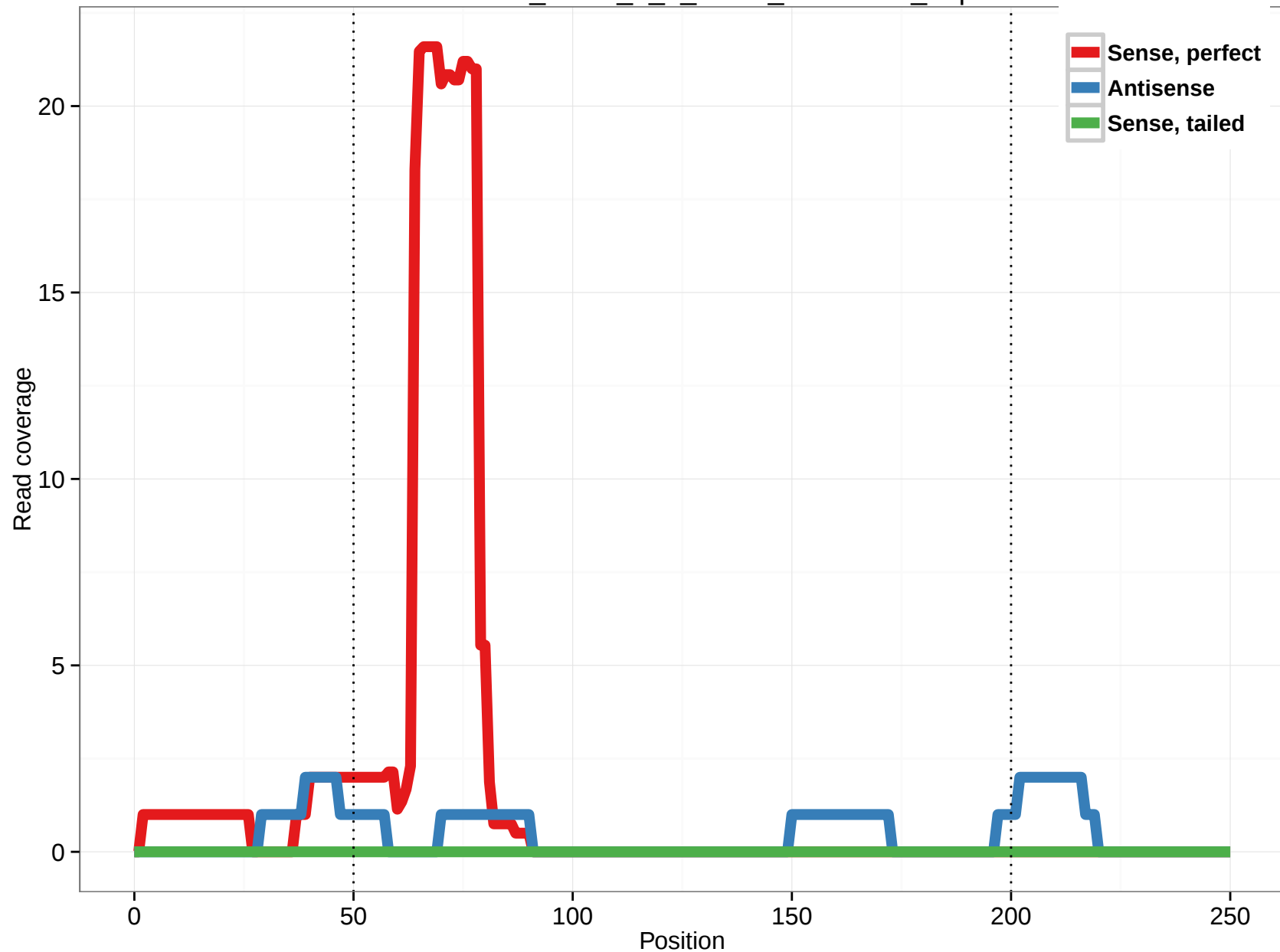
uc002abi.2_intron_1_0_chr15_52017319_r.5p
