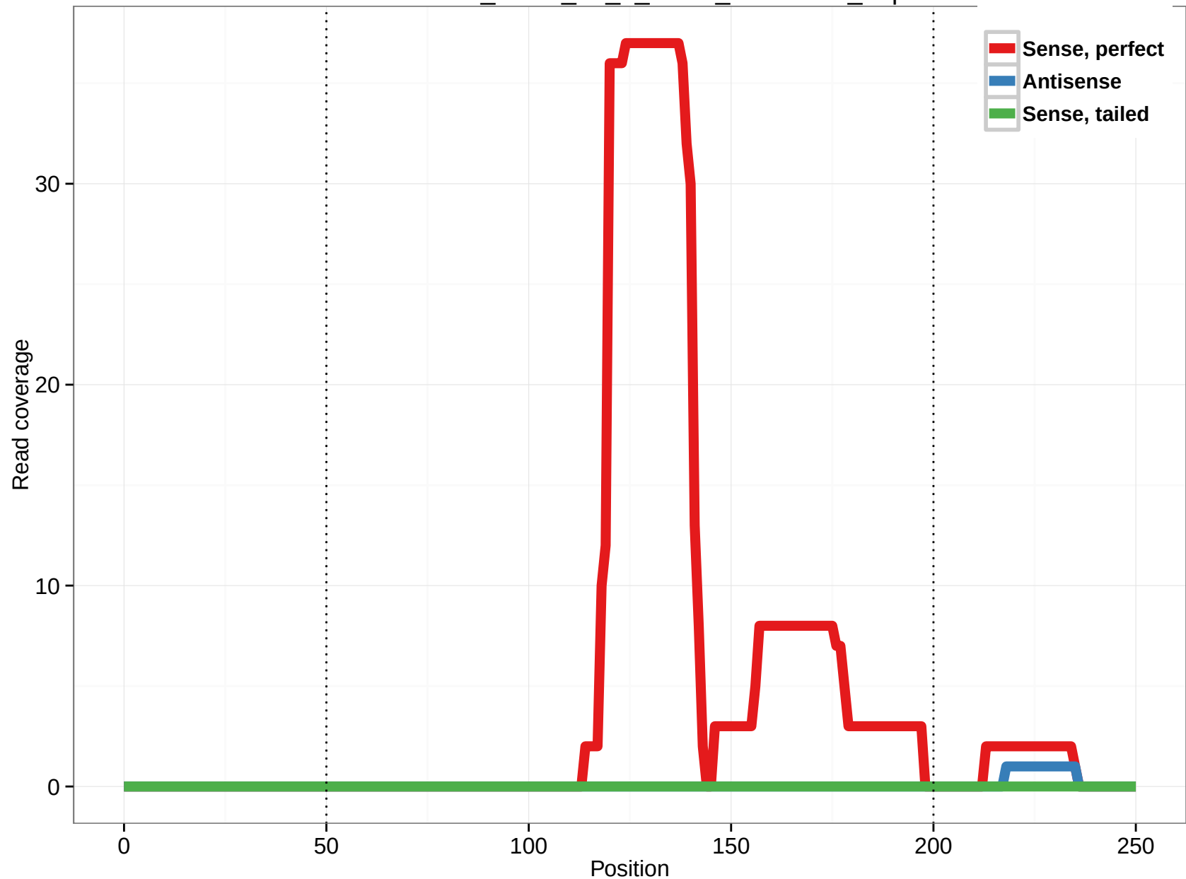
uc001zni.2_intron_30_0_chr15_41379881_r.3p
