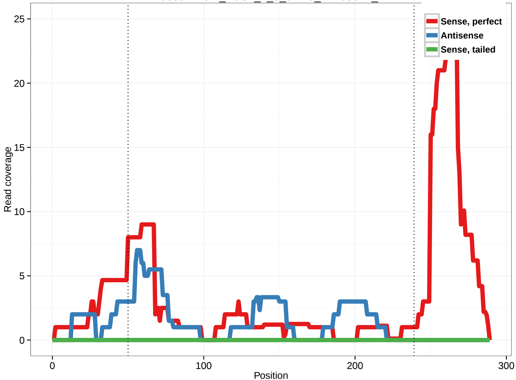
uc001znd.2_intron_1_0_chr15_41165941_r
