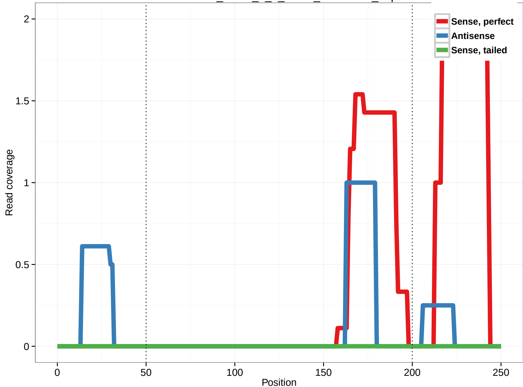
uc001zkl.2_intron_1_0_chr15_40231819_f.3p
