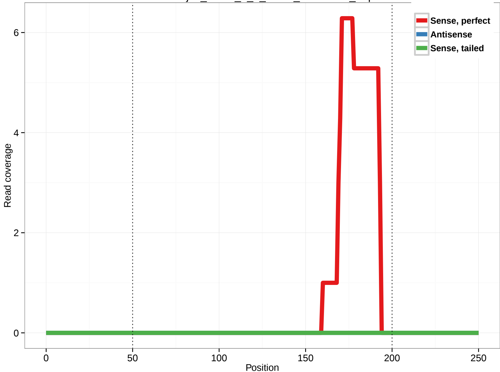
uc001zji.2_intron_4_0_chr15_37173870_r.3p
