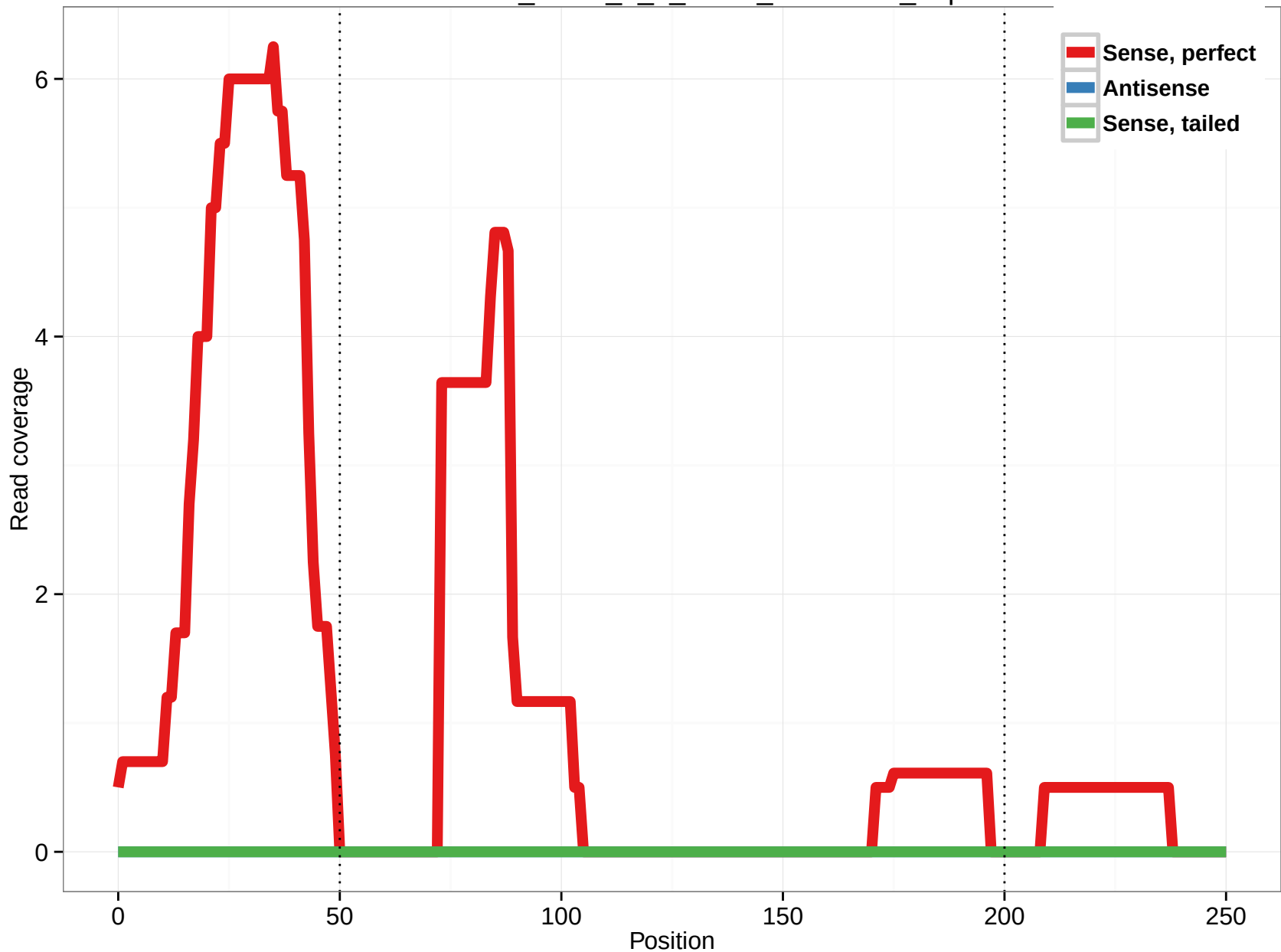
uc001zih.2_intron_8_0_chr15_34676249_r.5p
