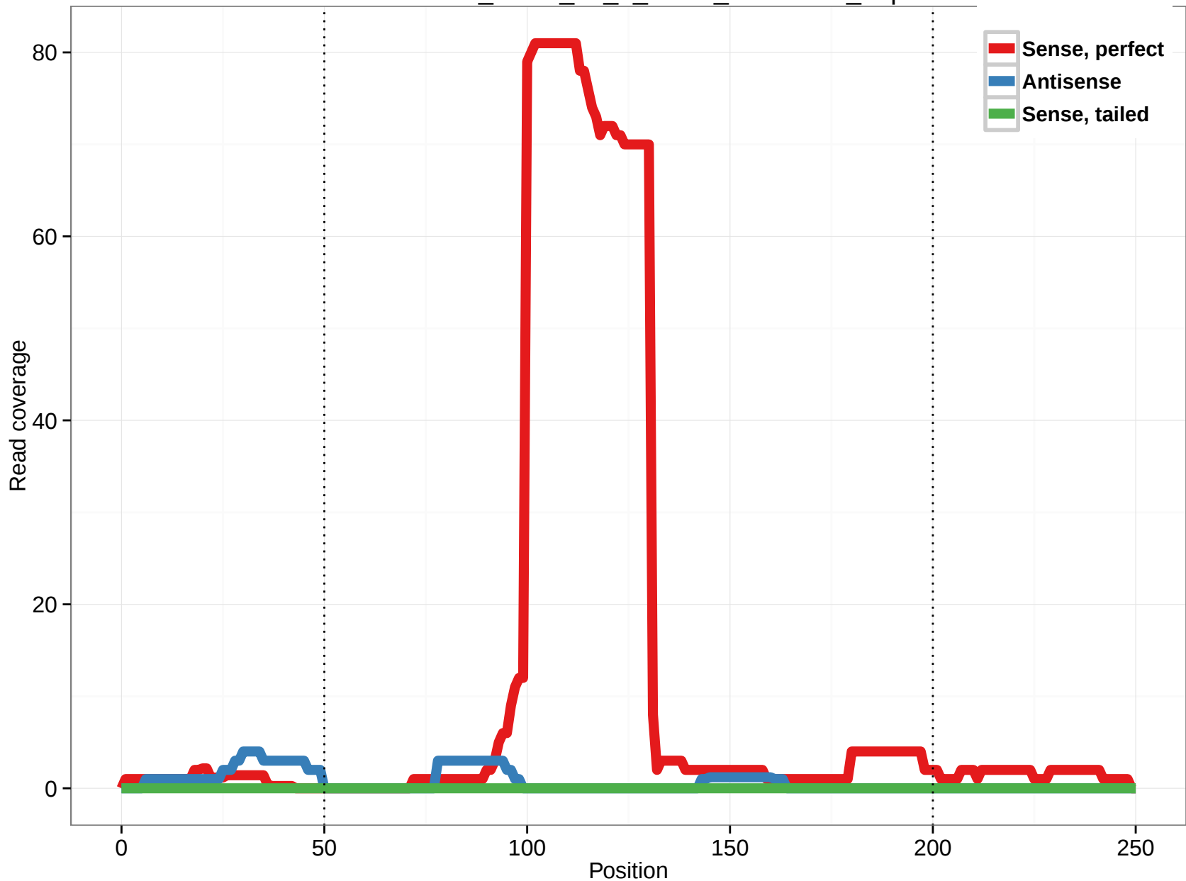
uc001zib.2_intron_24_0_chr15_34628869_r.5p
