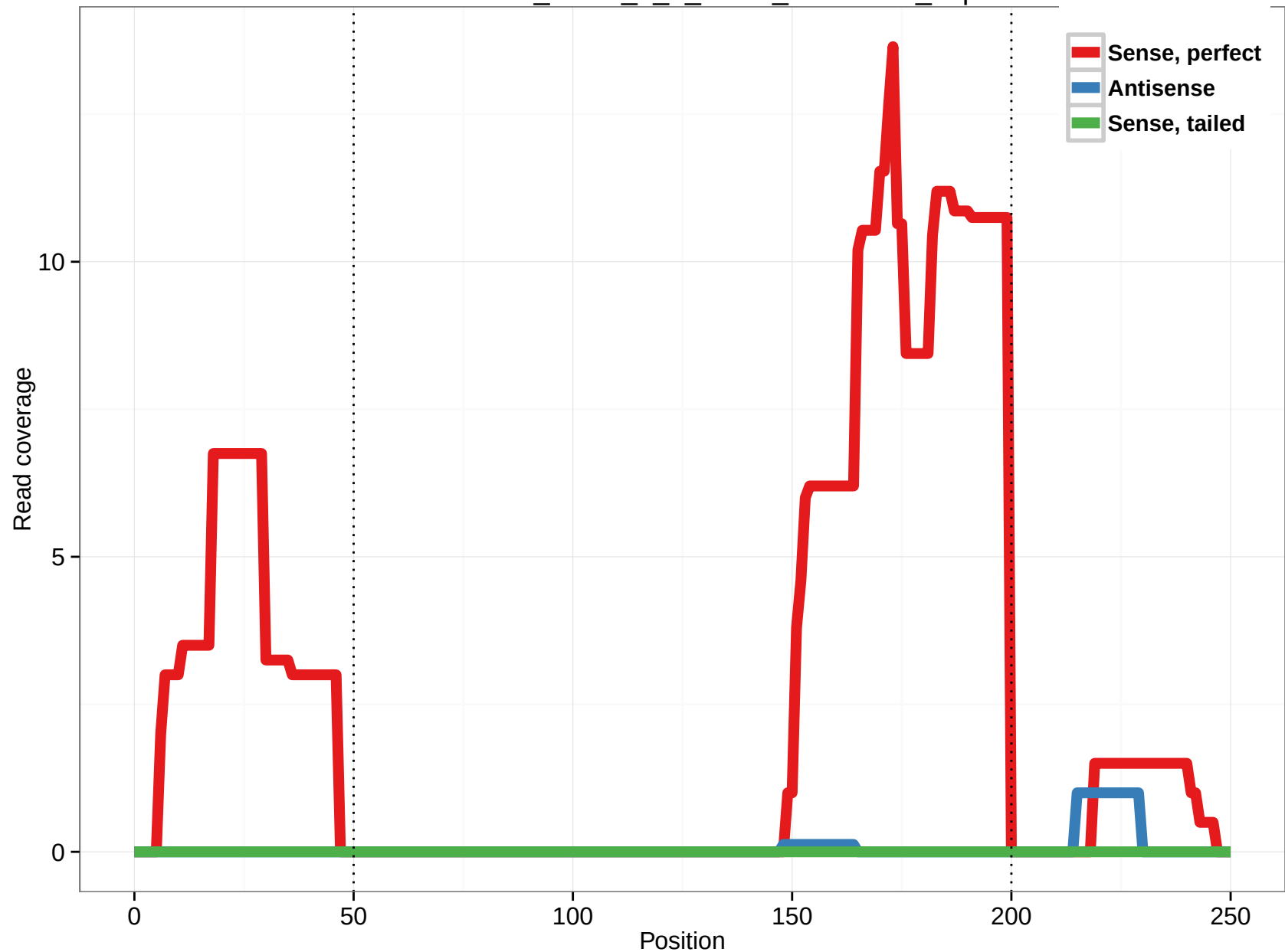
uc001zeu.2_intron_8_0_chr15_30938499_f.3p
