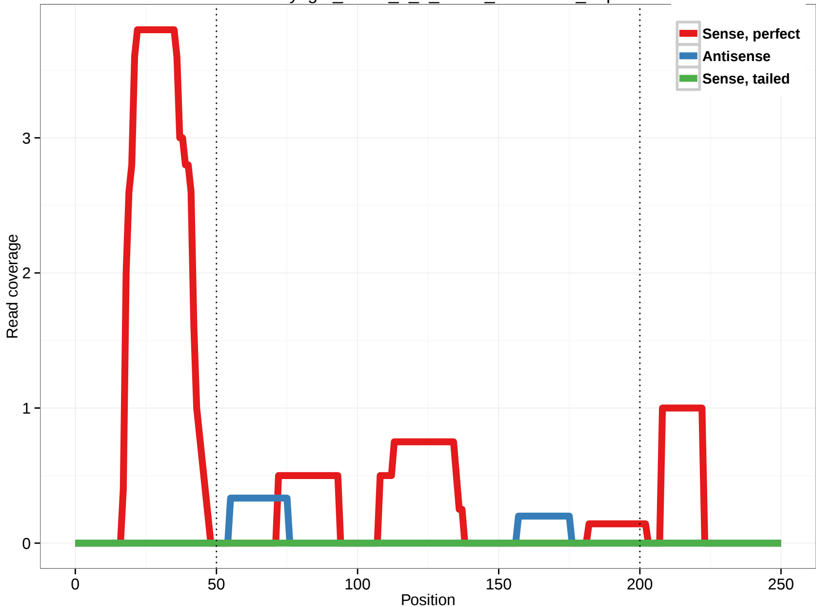
uc001yvg.2_intron_8_0_chr15_23201640_r.5p
