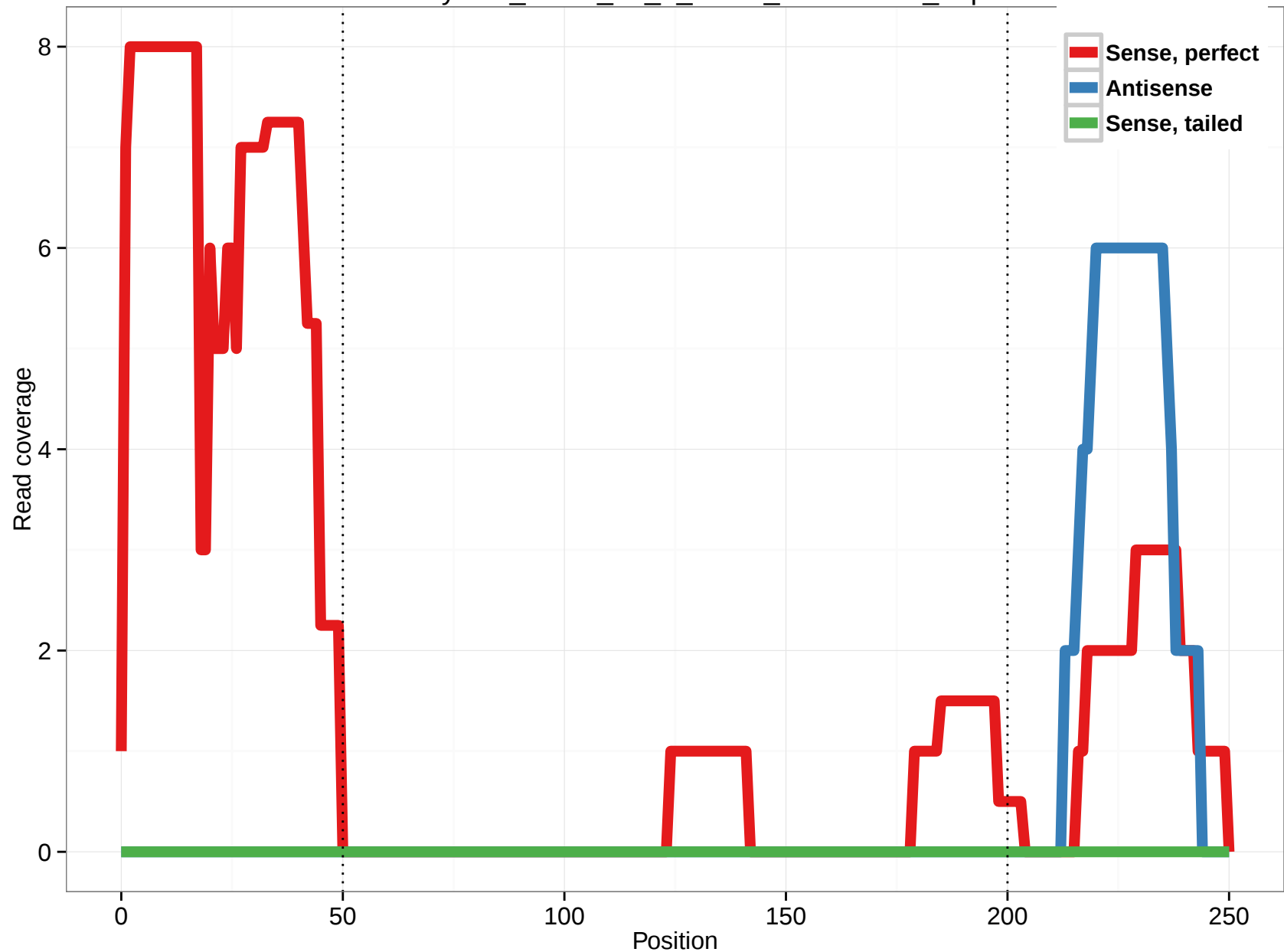
uc001ymi.1_intron_20_0_chr14_103433508_r.5p
