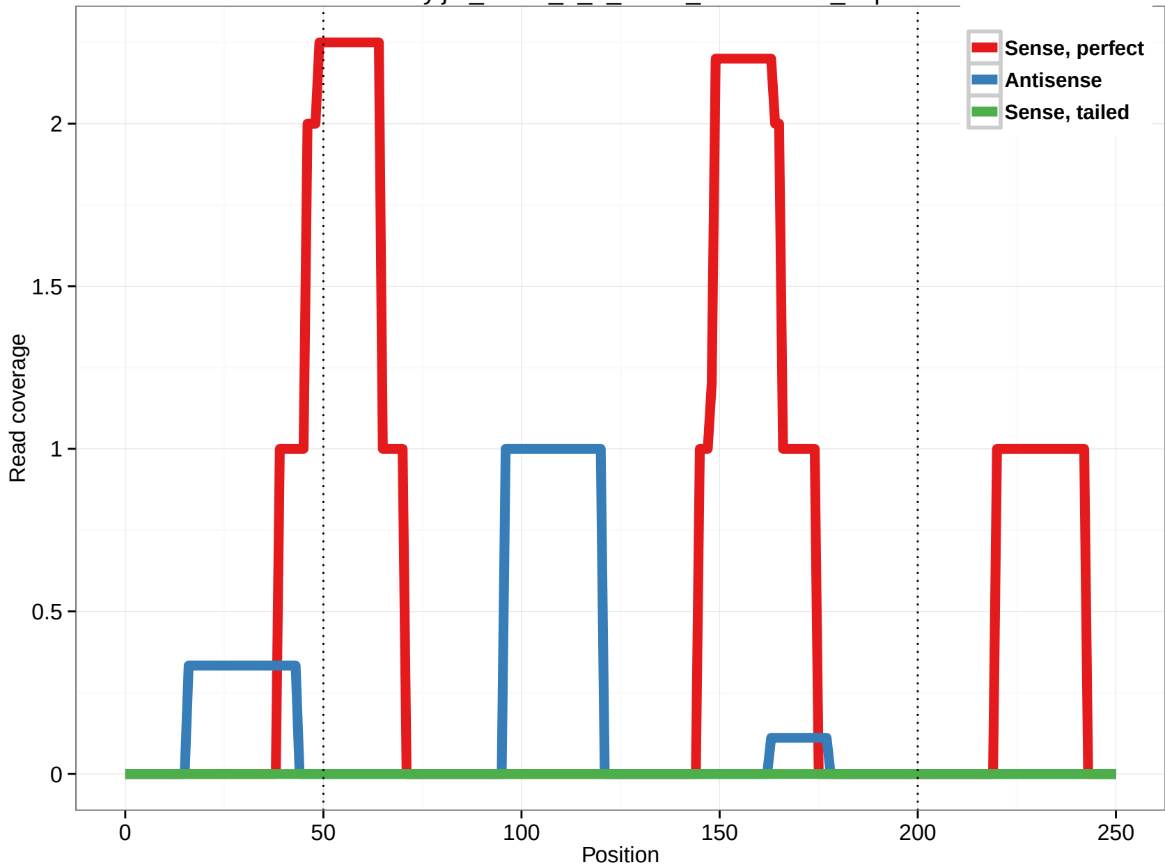
uc001ylj.2_intron_3_0_chr14_102700127_r.3p
