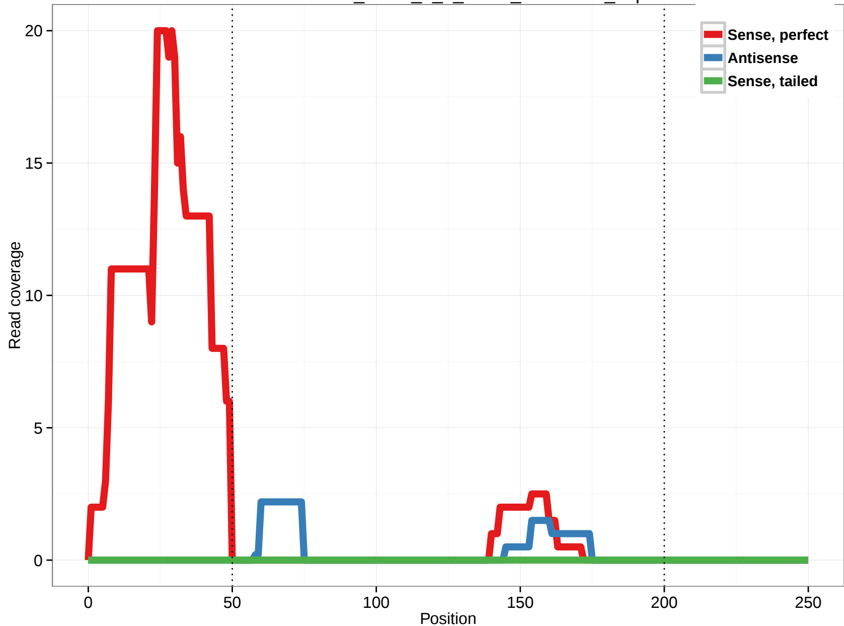
uc001xww.2_intron_7_0_chr14_89042285_f.5p
