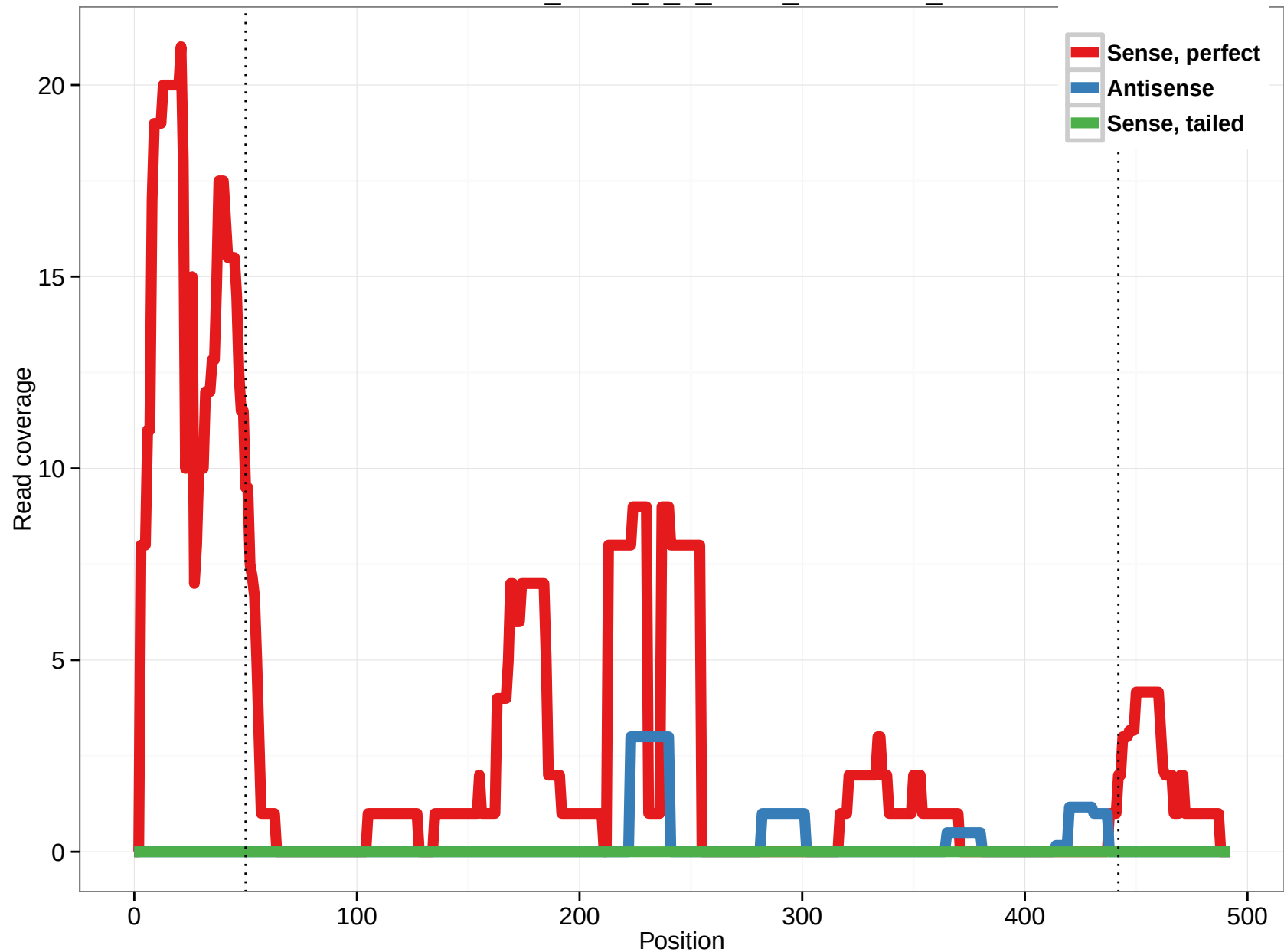
uc001xrf.2_intron_2_0_chr14_75530265_r
