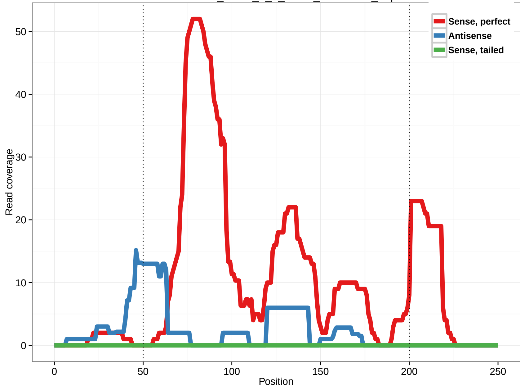
uc001xow.2_intron_0_0_chr14_74318647_f.5p
