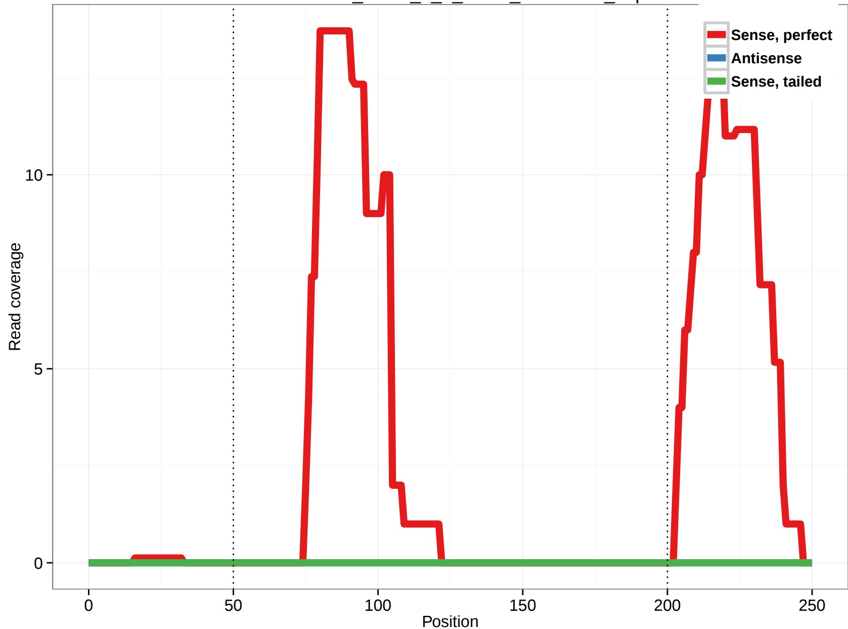
uc001xnn.3_intron_3_0_chr14_73544245_f.3p
