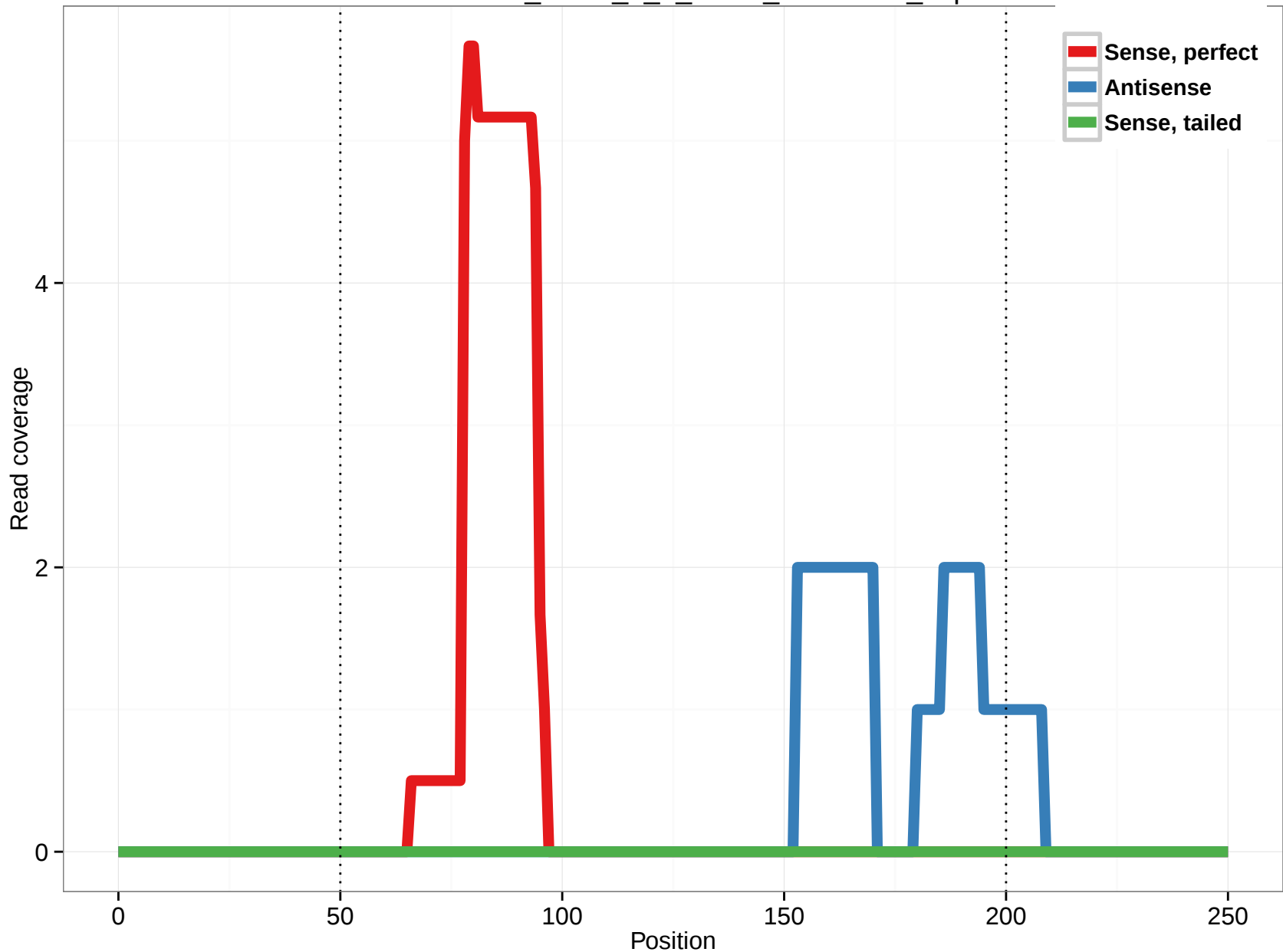
uc001xhd.3_intron_0_0_chr14_64932332_f.5p
