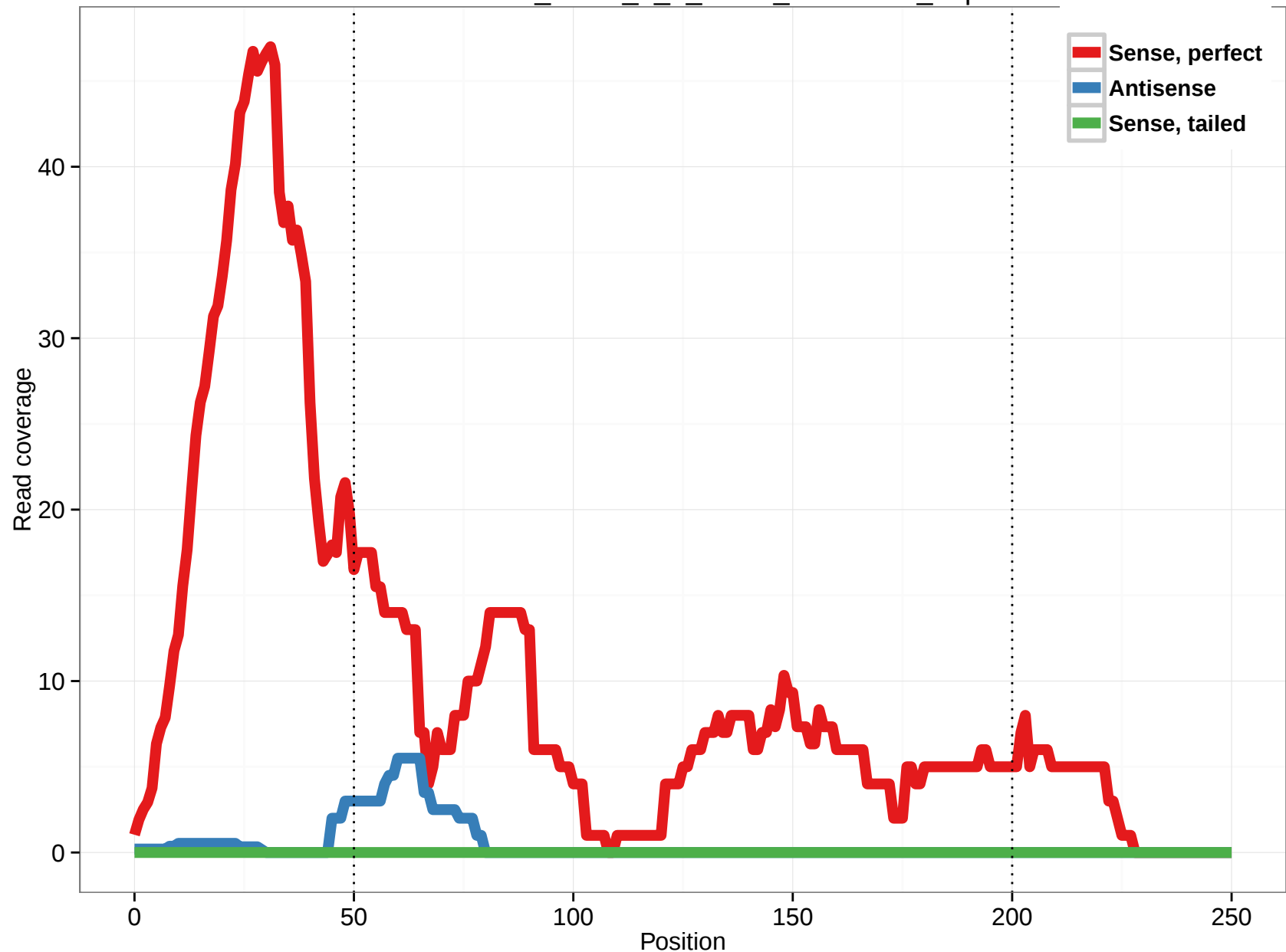
uc001wwl.2_intron_0_0_chr14_50044572_r.5p
