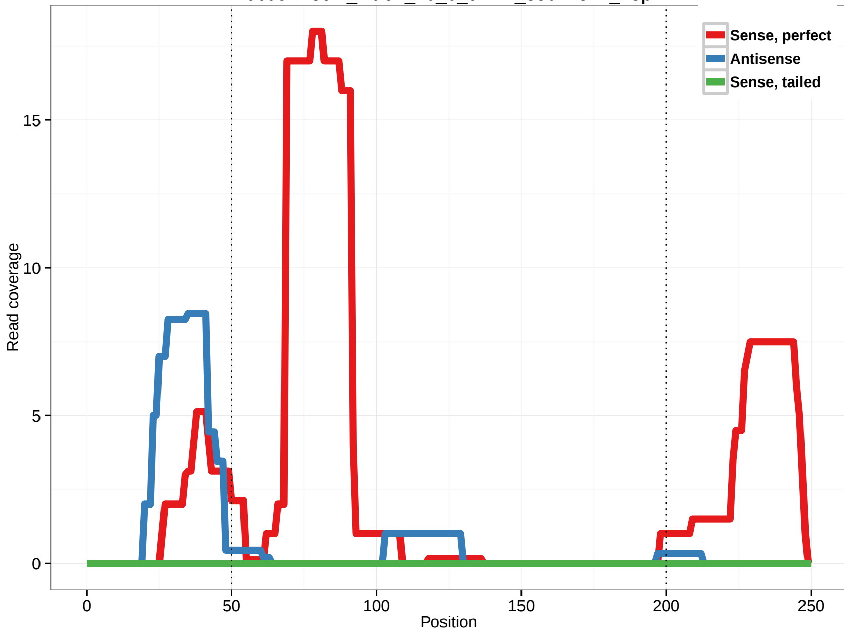
uc001wse.1_intron_10_0_chr14_35077347_r.3p
