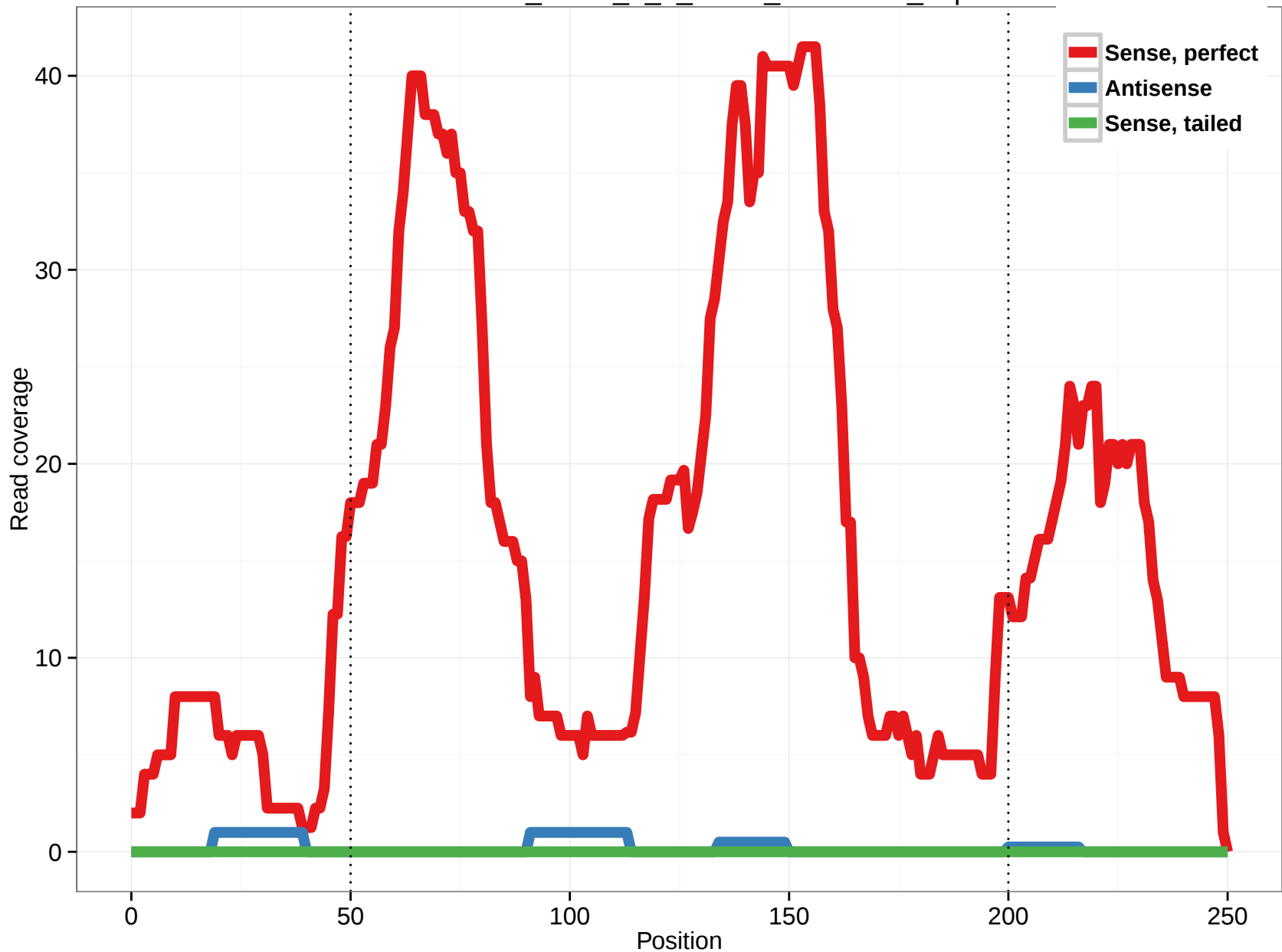
uc001wlr.1_intron_8_0_chr14_24572465_f.3p
