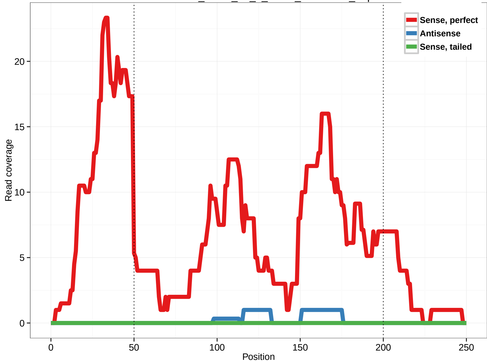
uc001wio.3_intron_10_0_chr14_23537881_r.5p
