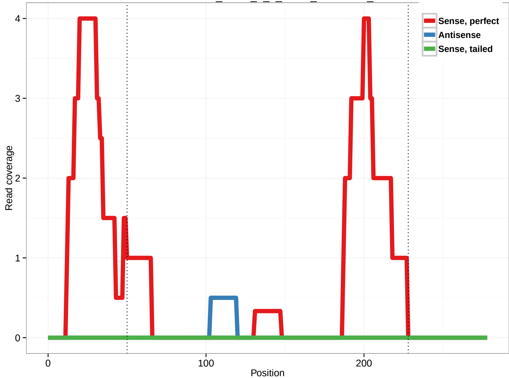
uc001war.1_intron_8_0_chr14_21863279_r
