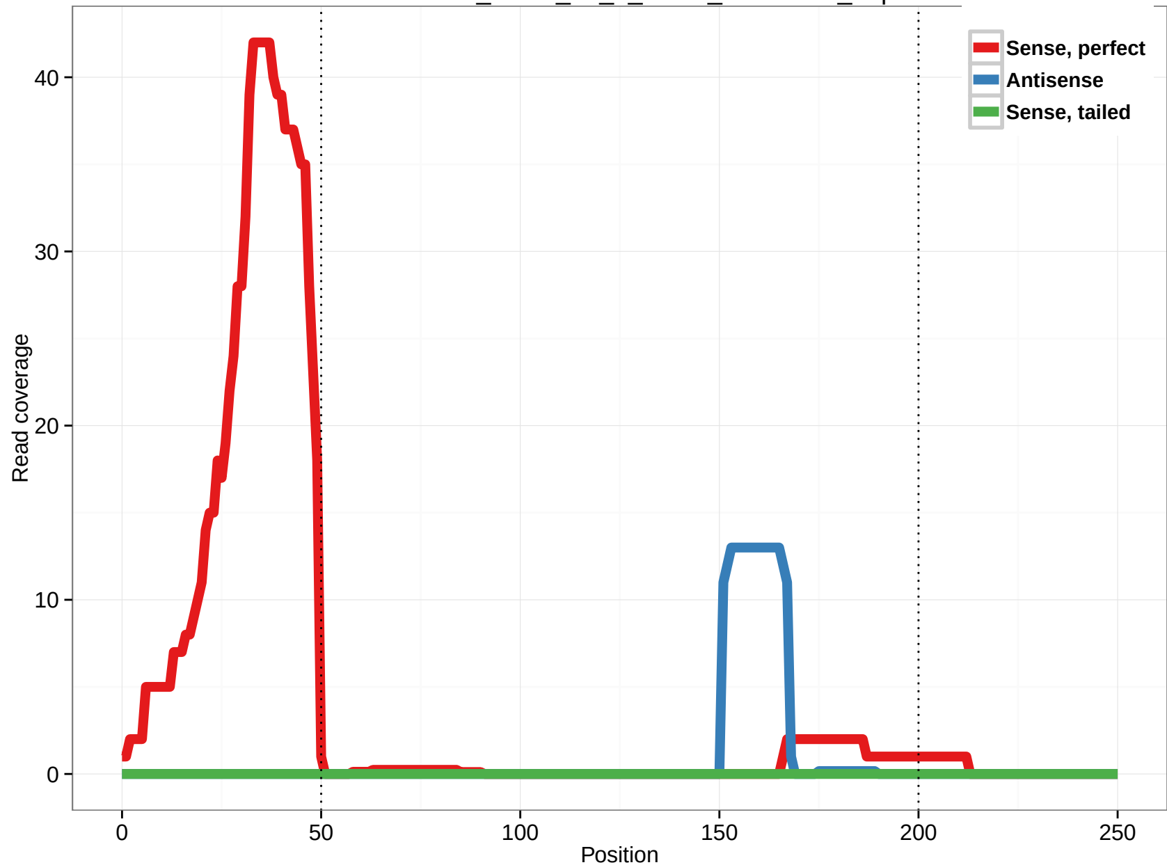
uc001war.1_intron_30_0_chr14_21883153_r.5p
