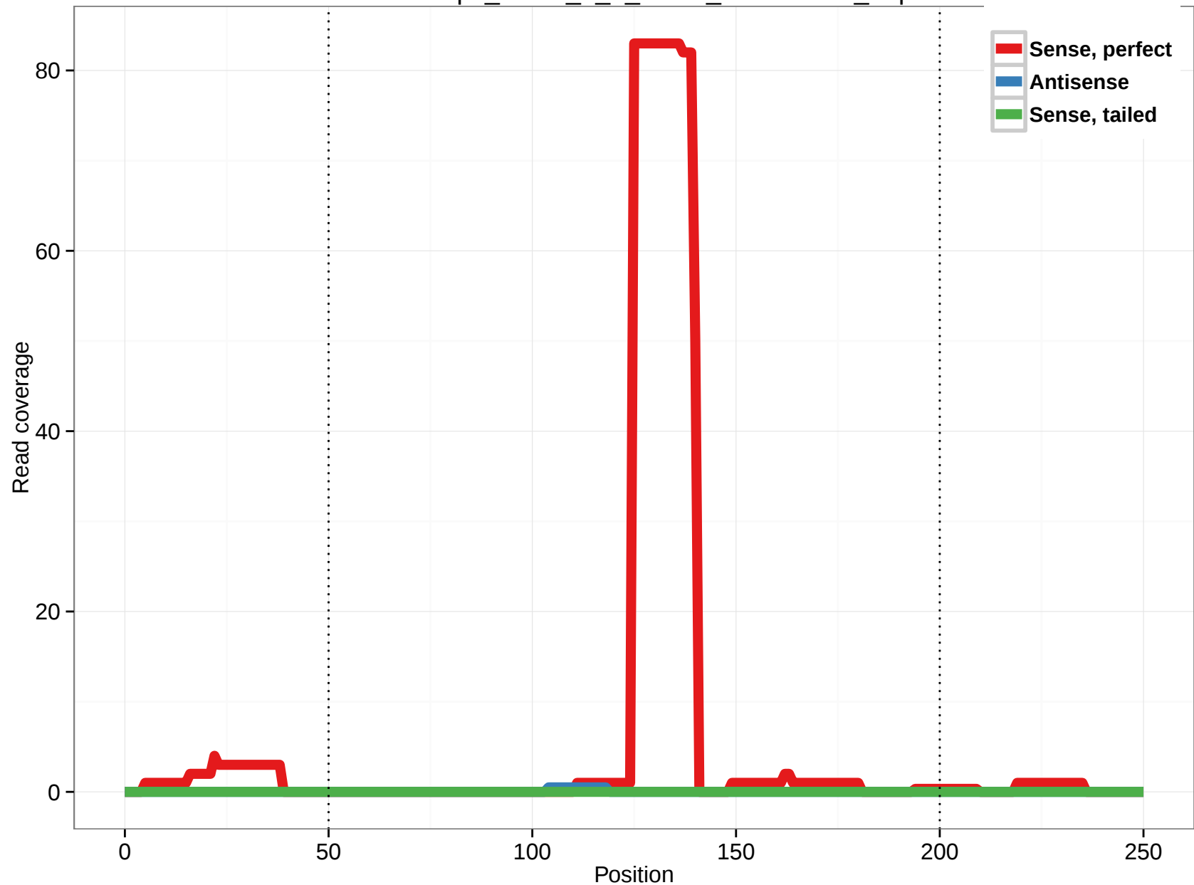
uc001vtq.1_intron_5_0_chr13_114098905_r.5p
