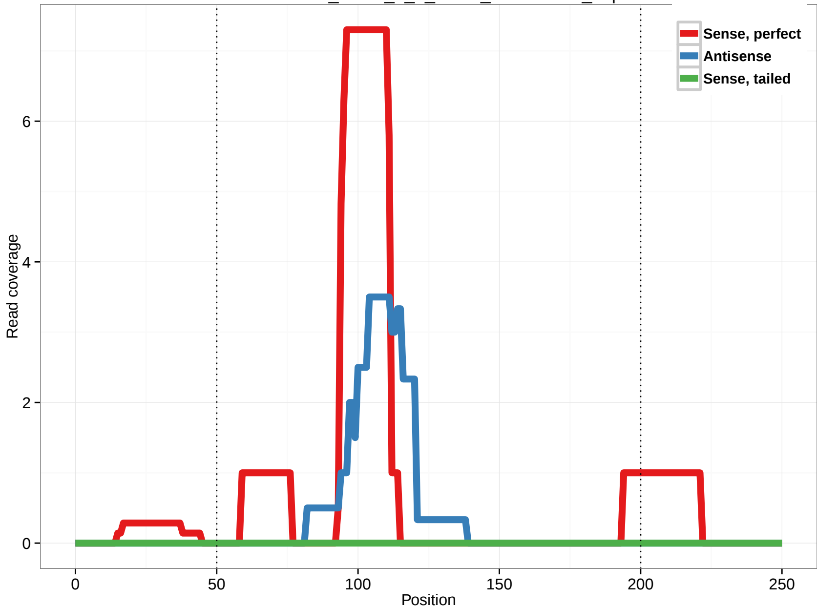
uc001vsh.1_intron_0_0_chr13_113301913_f.3p
