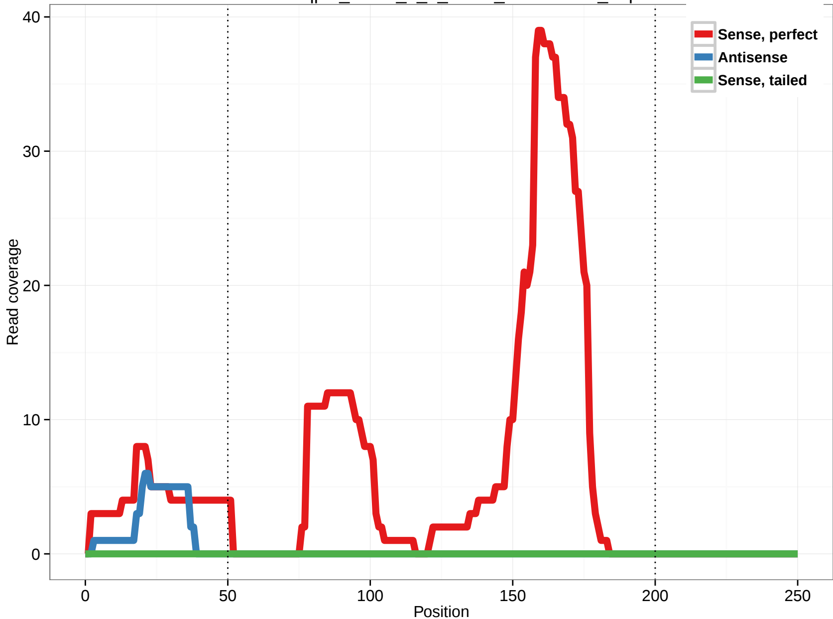
uc001vqp.2_intron_0_0_chr13_108863645_r.5p
