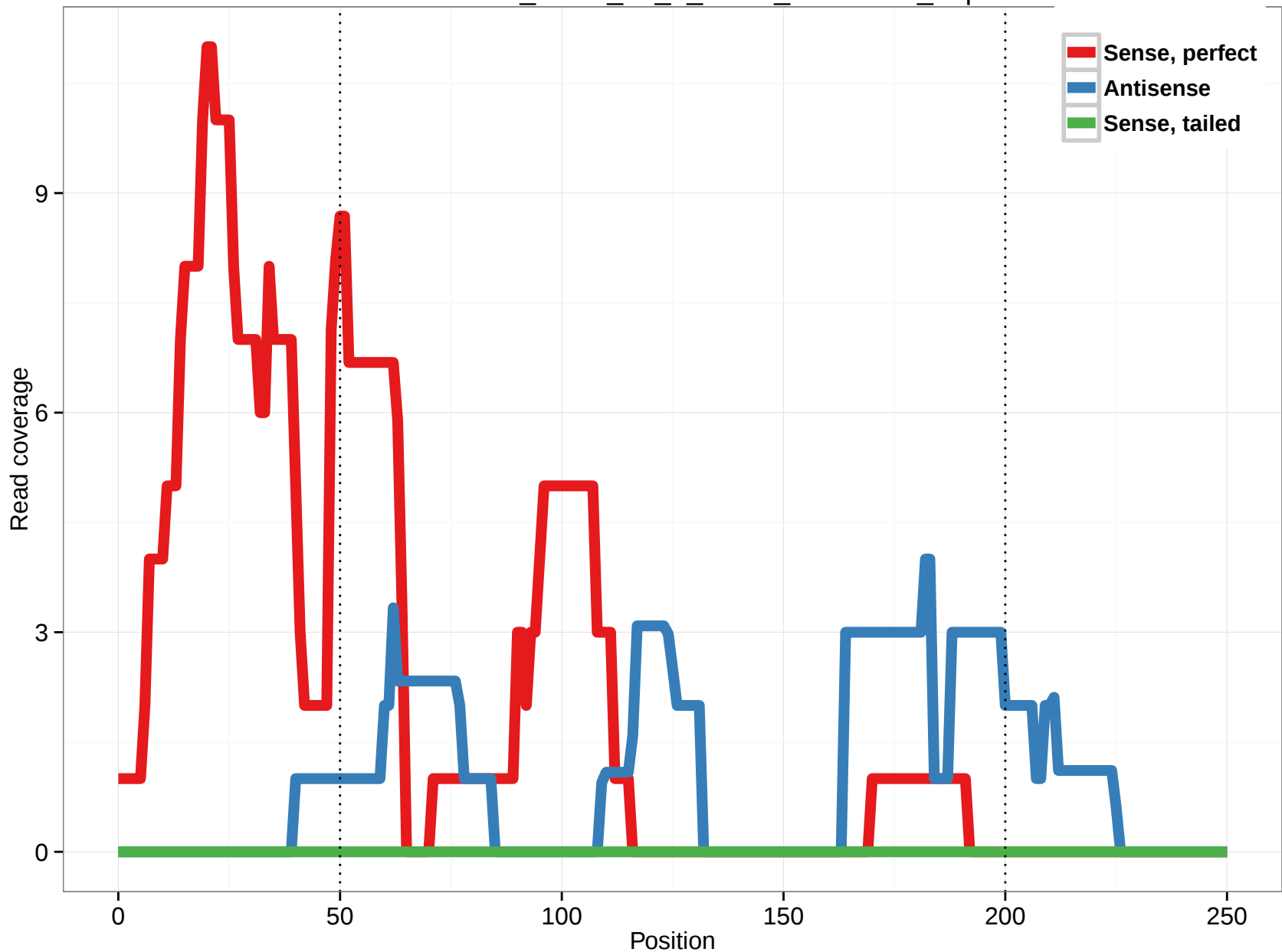
uc001vmd.3_intron_29_0_chr13_95900008_r.5p
