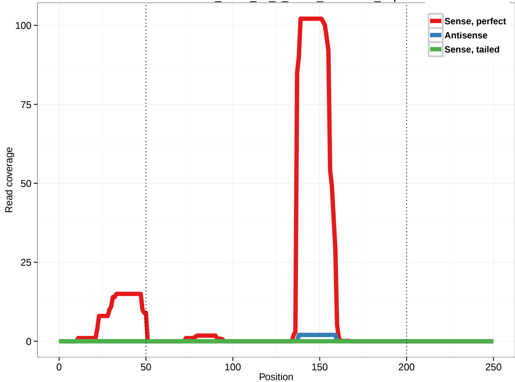
uc001vmd.3_intron_26_0_chr13_95863036_r.5p
