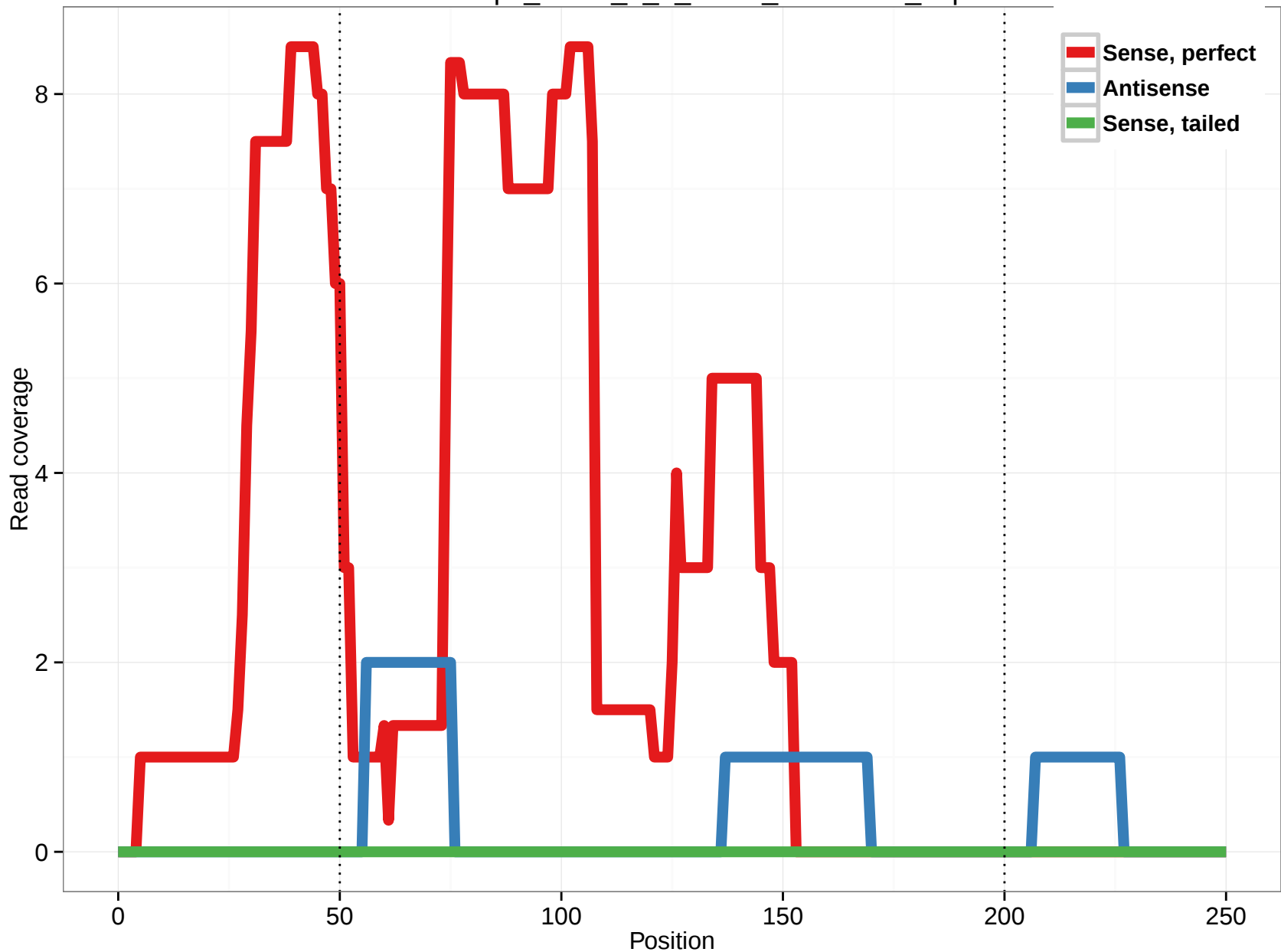
uc001vdq.1_intron_1_0_chr13_50571900_f.5p
