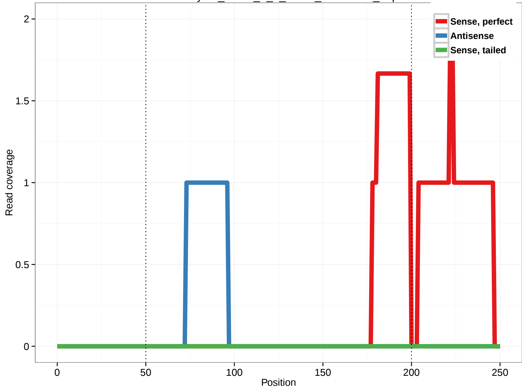
uc001uys.1_intron_7_0_chr13_42878000_f.3p
