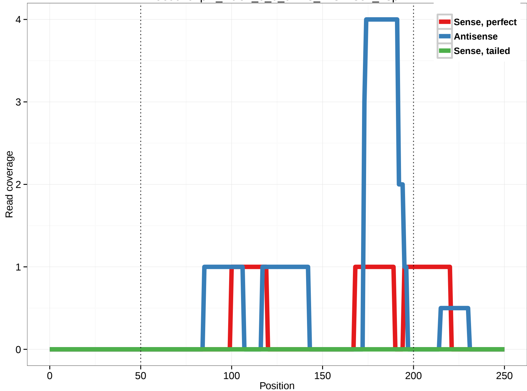
uc001uxp.1_intron_0_0_chr13_41374861_r.3p
