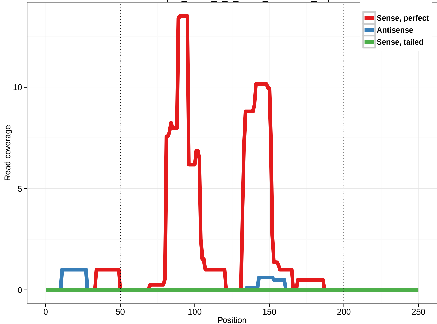
uc001uqk.2_intron_0_0_chr13_25946427_f.5p
