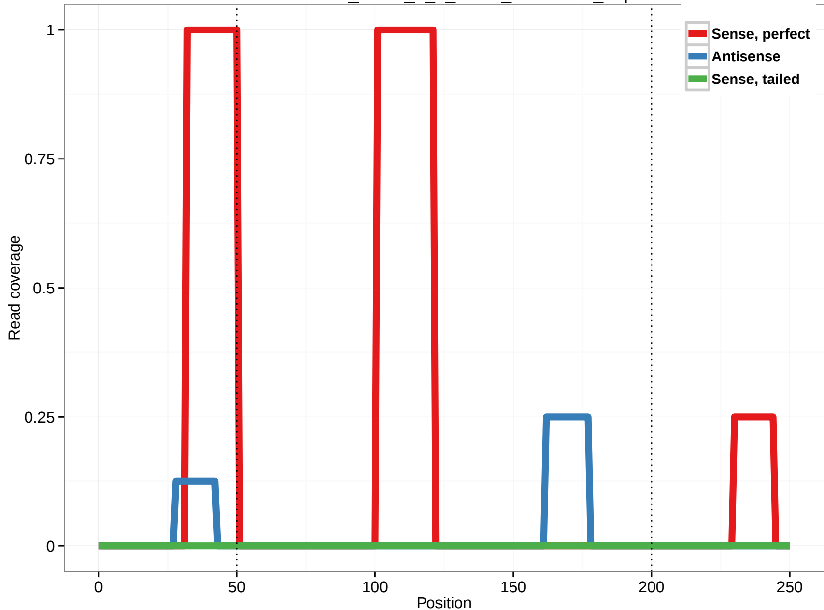
uc001uox.3_intron_1_0_chr13_24330758_r.5p
