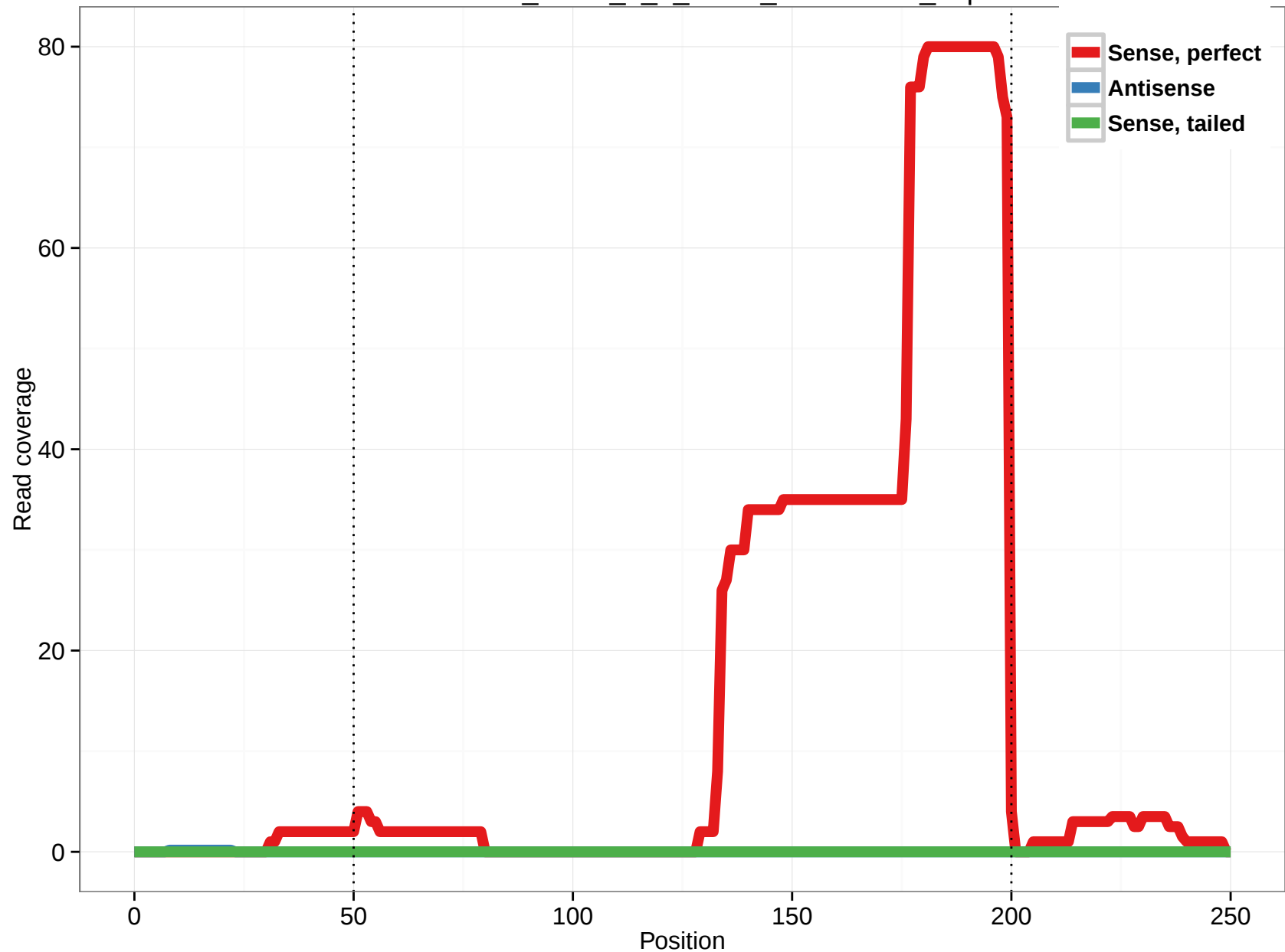
uc001ufz.2_intron_3_0_chr12_124489483_f.3p
