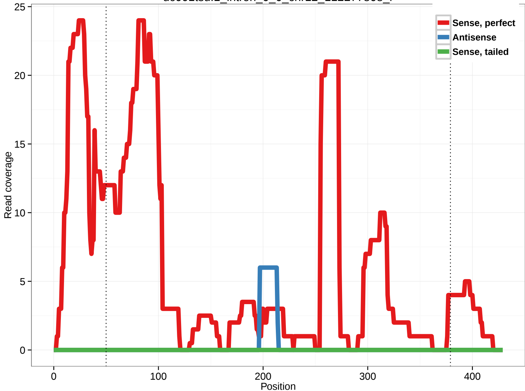
uc001tsu.1_intron_0_0_chr12_112277808_r
