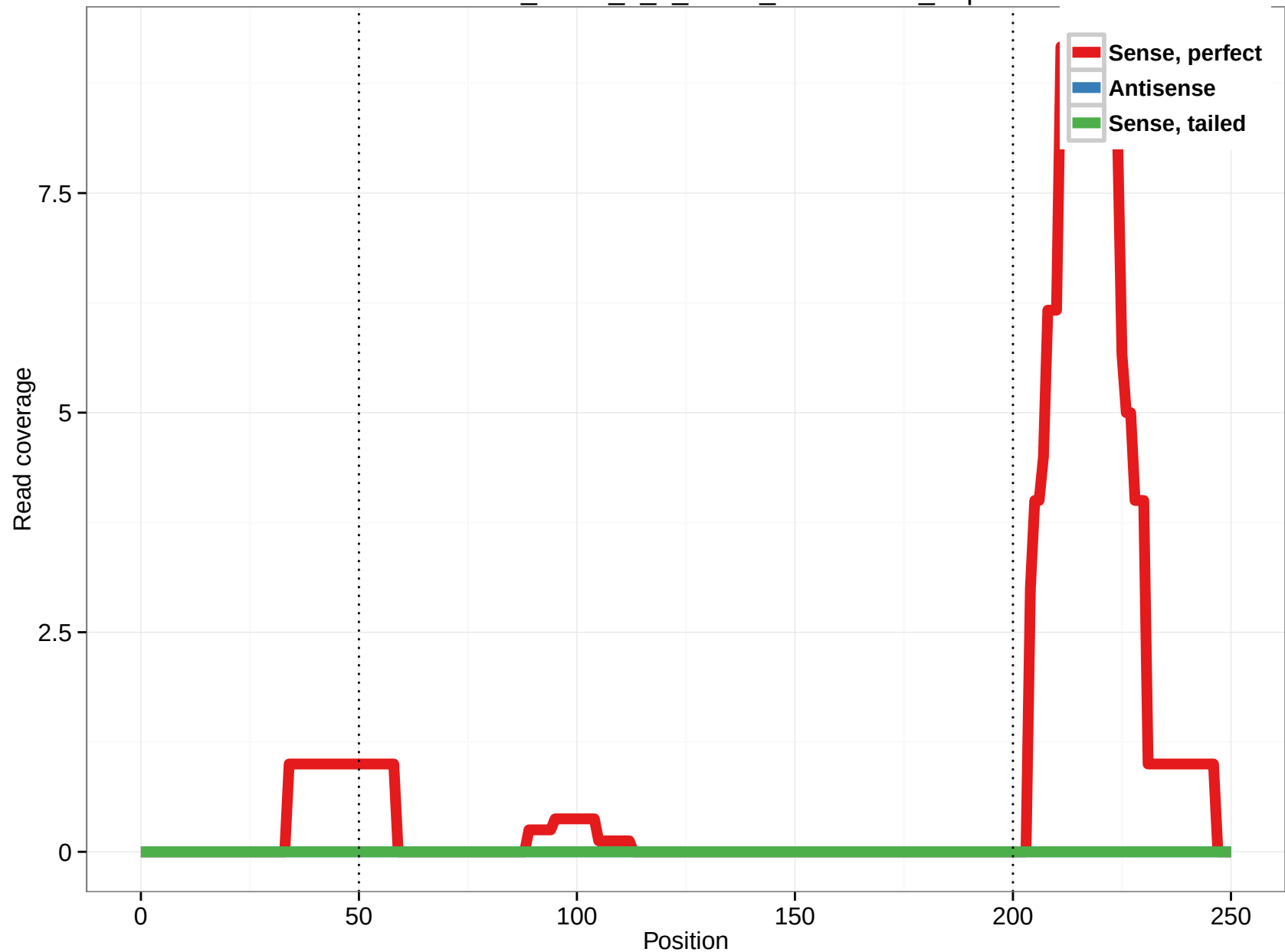
uc001tla.2_intron_7_0_chr12_105289124_r.3p
